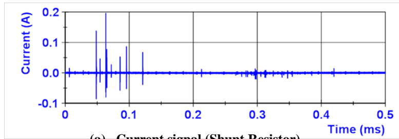
(a) Current signal (Shunt Resistor)
