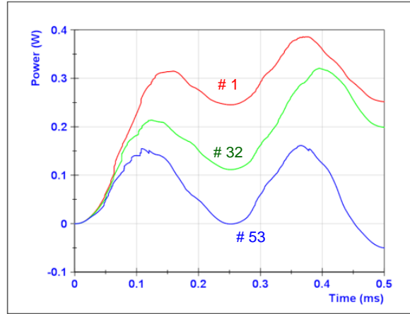
(b) Resistor Method - Cycles No. 1, 32, 53
