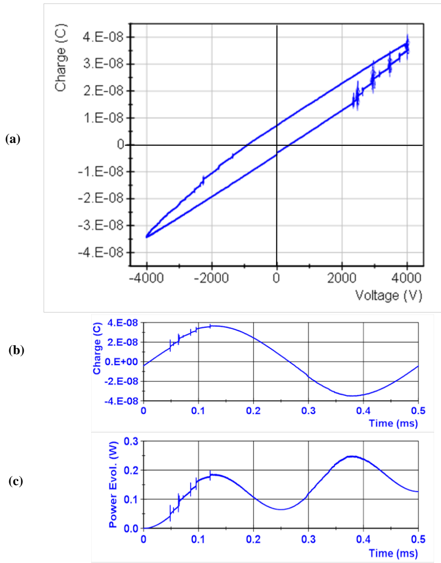
Figure 12. Monitor Capacitor method (a) Lissajous Curve, (b) Capacitor charge signal, (c) Average power evolution
