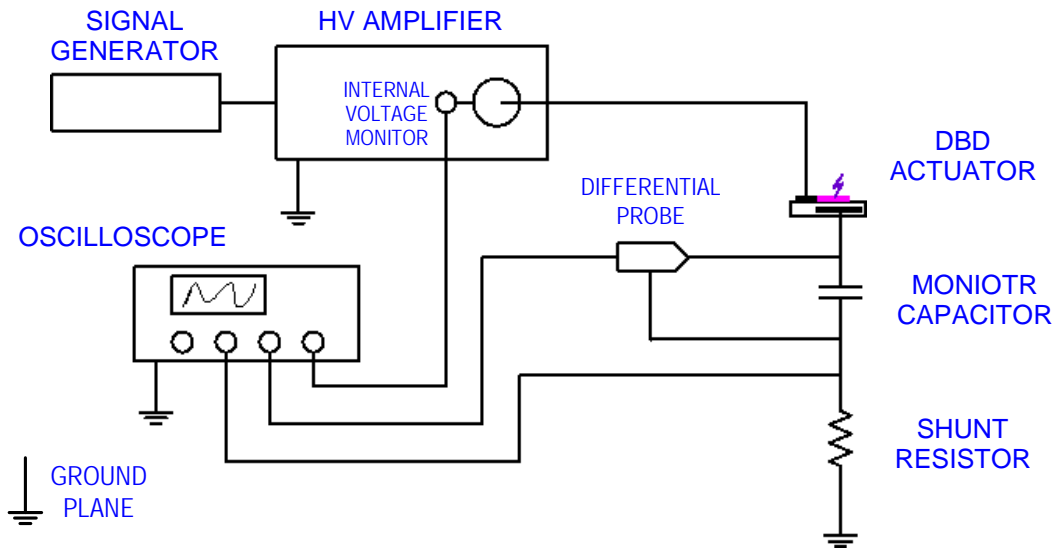
Figure 6. Schematic of the test setup
