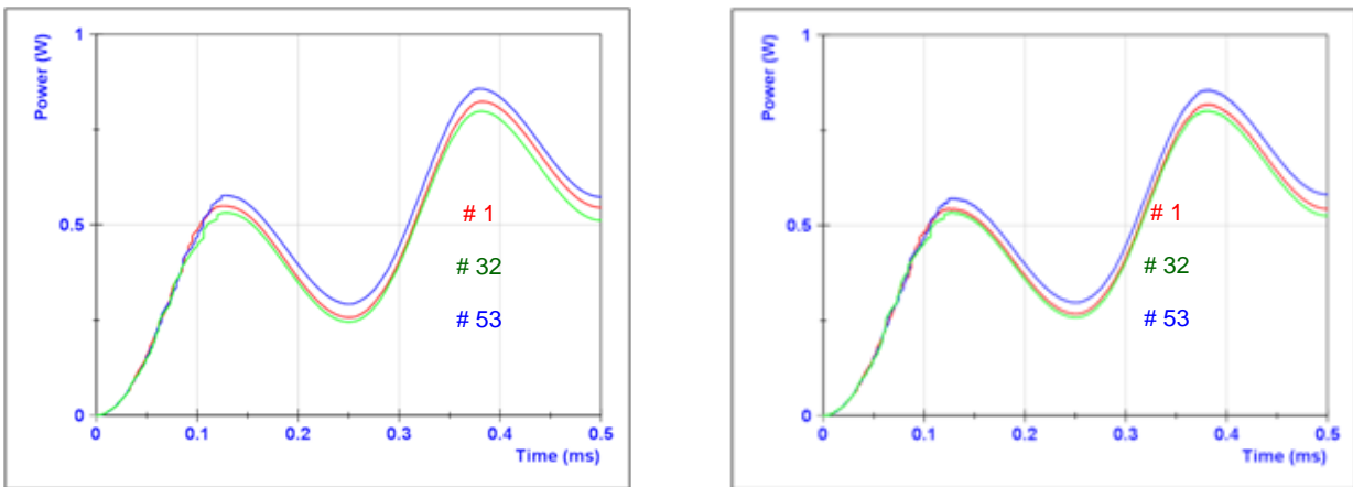
(a) Resistor method with Compression
