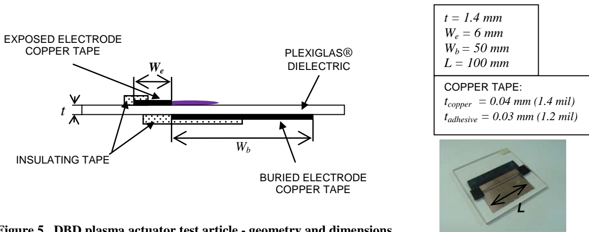
Figure 5. DBD plasma actuator test article - geometry and dimensions.
