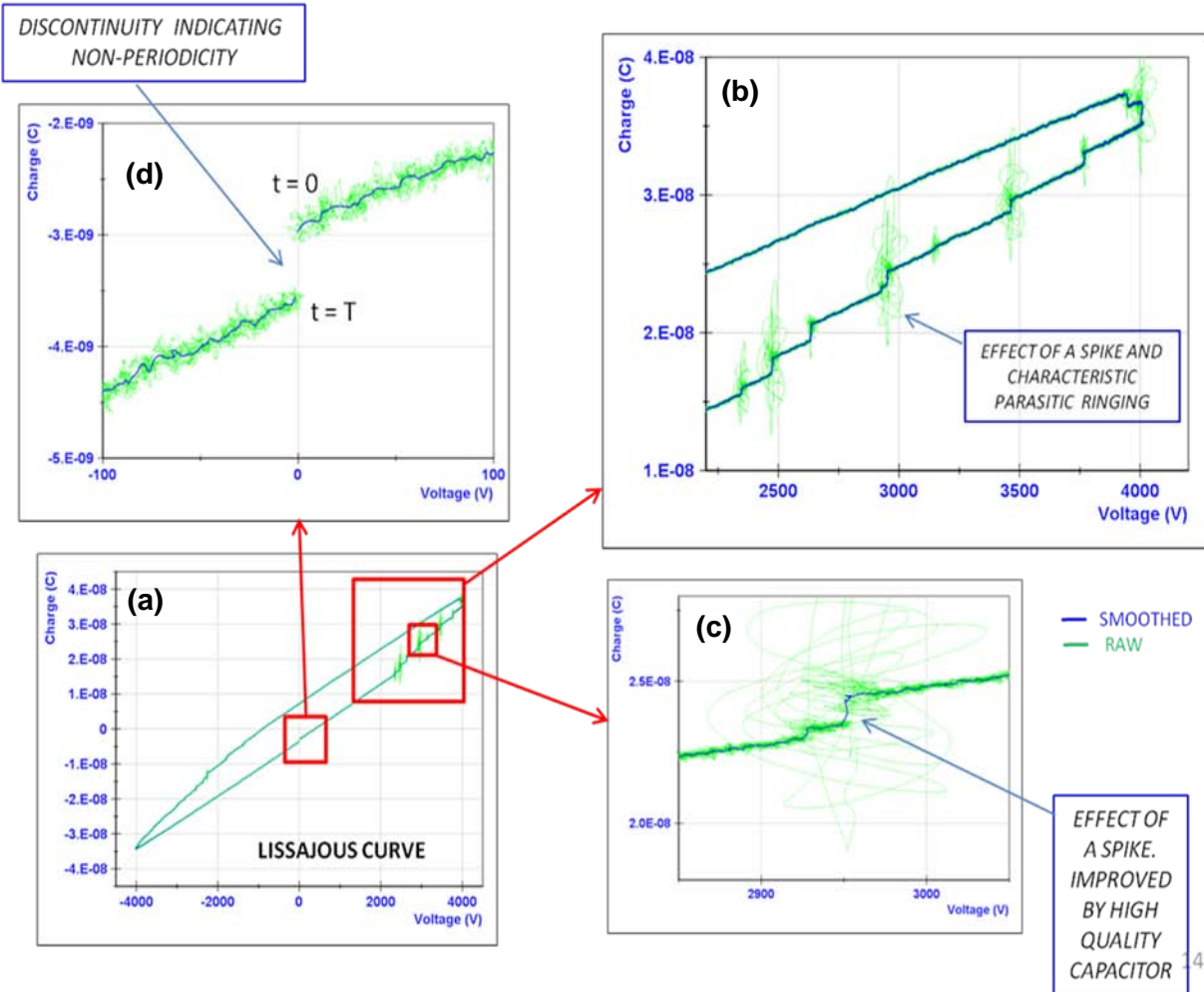
Figure 16. Lissajous Curve - detail (a) Full-scale curve (b) Enlargement of the backward stroke region (c) Enlargement of an individual spike trajectory (d) Enlargement of cycle-end discontinuity. Green- Raw data, Blue – Smoothed data
