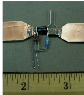
(c) Compression circuit attached to monitor capacitor and shunt resistor.
