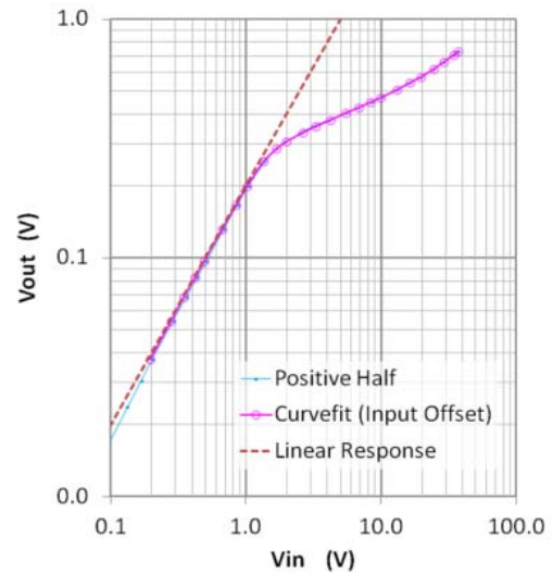
(b) Diode compression circuit transfer function (Purple). Straight line (Red) is linear for reference.
