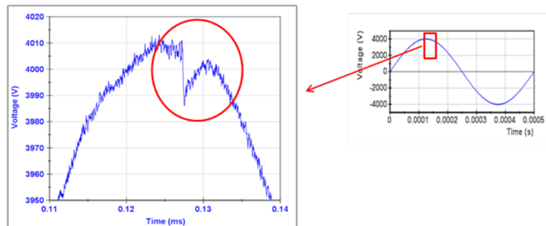
Figure 13. Applied Voltage - detail
