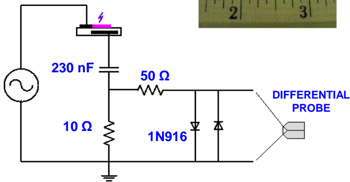
(a) Schematic of two-diode compression circuit.
