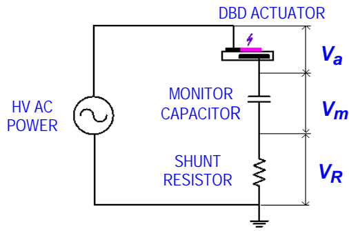
Figure 4. Circuit for simultaneous monitor capacitor and shunt resistor methods.
