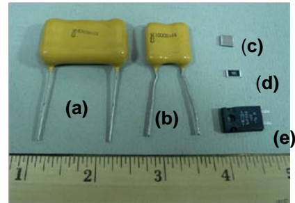
Figure 8. Capacitors and resistors used: (a), (b) Mica capacitors (c) Chip capacitor (d) Chip resistor (e) Metal film resistor in TO-220 case.
