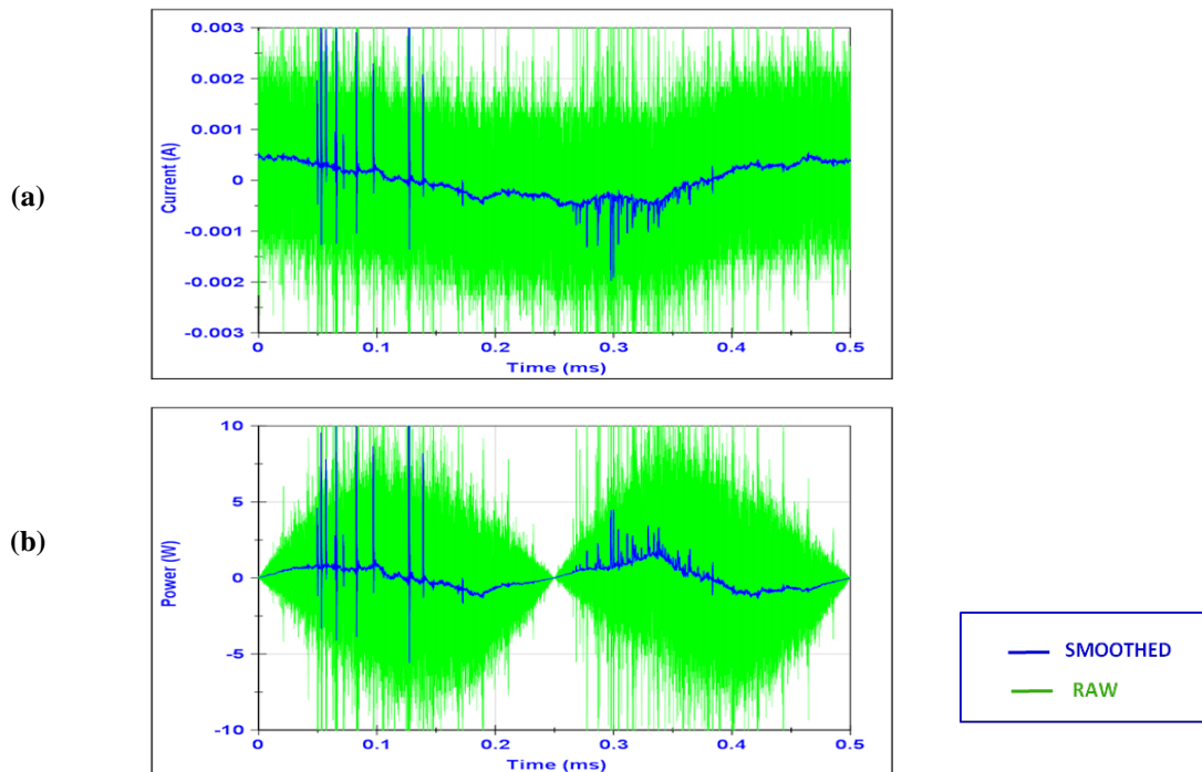
Figure 15. Visual Noise Reduction with smoothing (a) Current, (b) Instantaneous Power.
