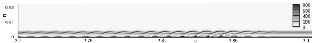
Figure 13. Nonlinear development of 475 kHz second mode instability for conditions at 21.5 seconds into the flight. Flood contours show the normal density gradient in the presence of large amplitude second mode waves. The coordinates s and n correspond to the distance from the nose tip along the cone surface and the wall normal coordinate, respectively. Both coordinates are measured in feet in this figure.
