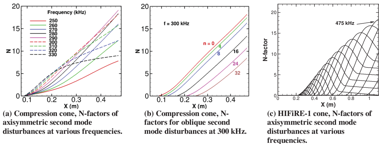
Figure 2. Linear N-factors of second mode disturbances for cone models of interest
