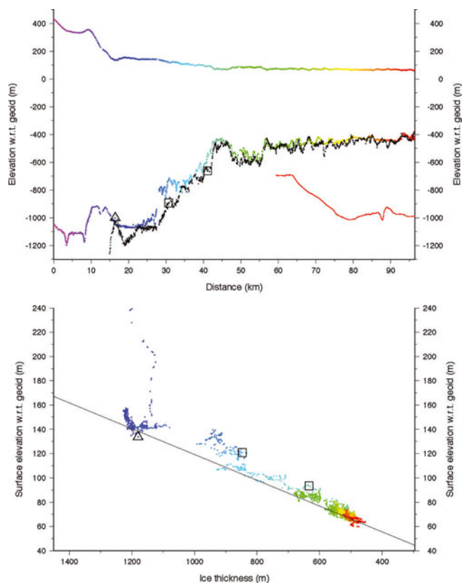
Fig. 6. Airborne data along profile 3 (cf. Fig. 1). Same as Figure 4 and open squares indicate locations from Figure 2 where flight-line crosses the 1992 grounding line.
