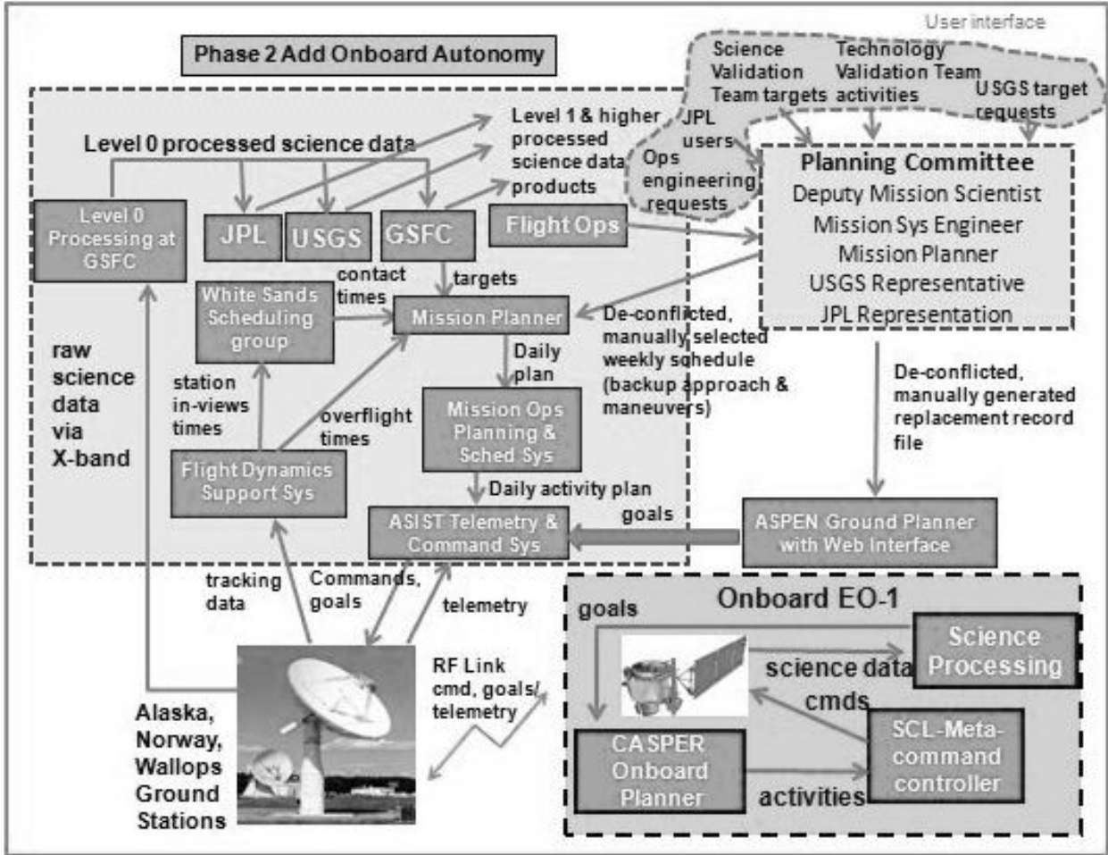
Fig. 2. In phase 2, onboard autonomy software was added which reduced the effort for planning and thus the planning committee reduced their meetings to once a week
