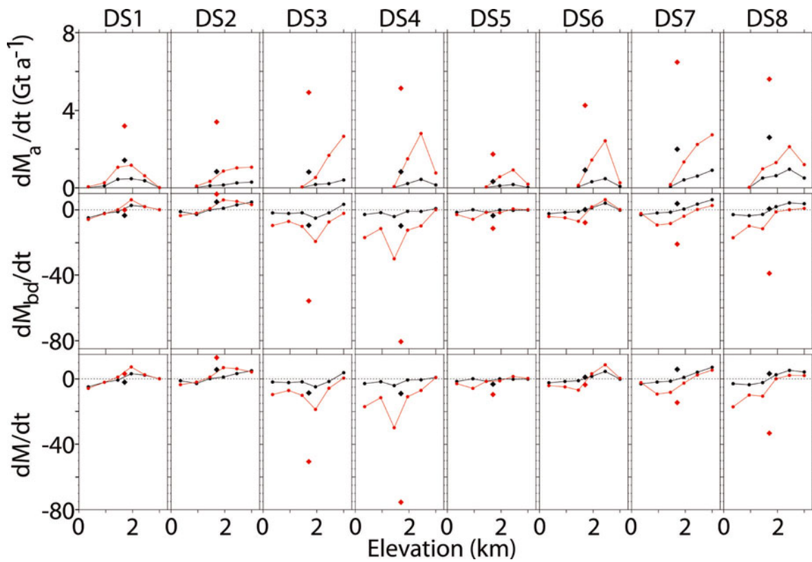
Fig. 12. Components of mass change by drainage system. dM_a/dt , dM_{bd}/dt , dM/dt ( Gt a^{-1} ) averaged over 500 m elevation bands for the eight drainage systems for 1992–2002 (black) and 2003–07 (red) with totals for 1992–2002 (black symbols) and 2003–07 (red symbols). Accumulation-driven mass increases are largest in DS3, DS4, DS7 and DS8, and dynamic-/ablation-driven thinning is largest in DS3, DS4 and DS8 and very small in DS1, DS2, DS5 and DS6.
