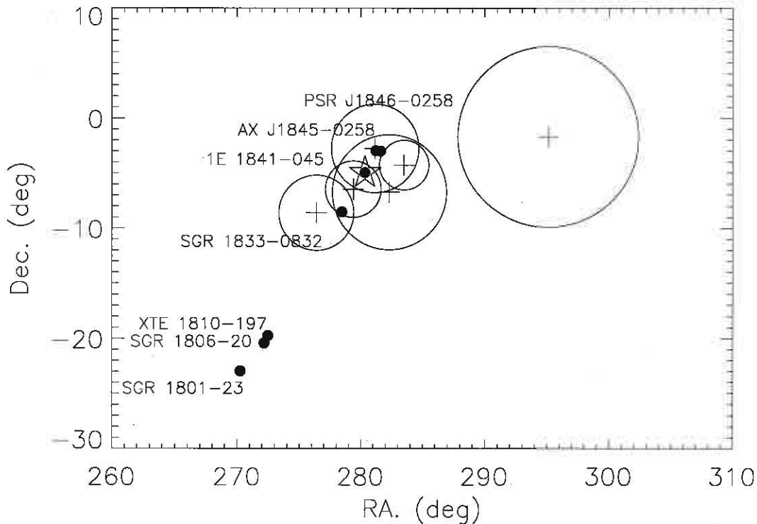
Fig. 1.— Locations of the four BAT bursts ( star ) and 6 GBM bursts ( crosses ) with 1\sigma error circle. The Chandra location of 1E 1841-045 ( filled dot within the star ), and 6 other nearby magnetar candidates are also indicated ( filled dots ).
