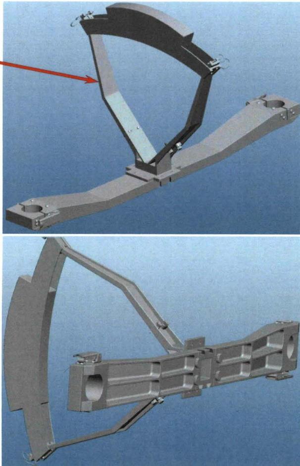
Center hub
