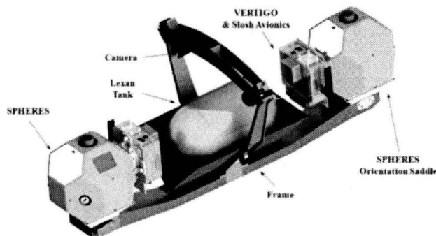
Figure 1 SPHERES Slosh Experiment
