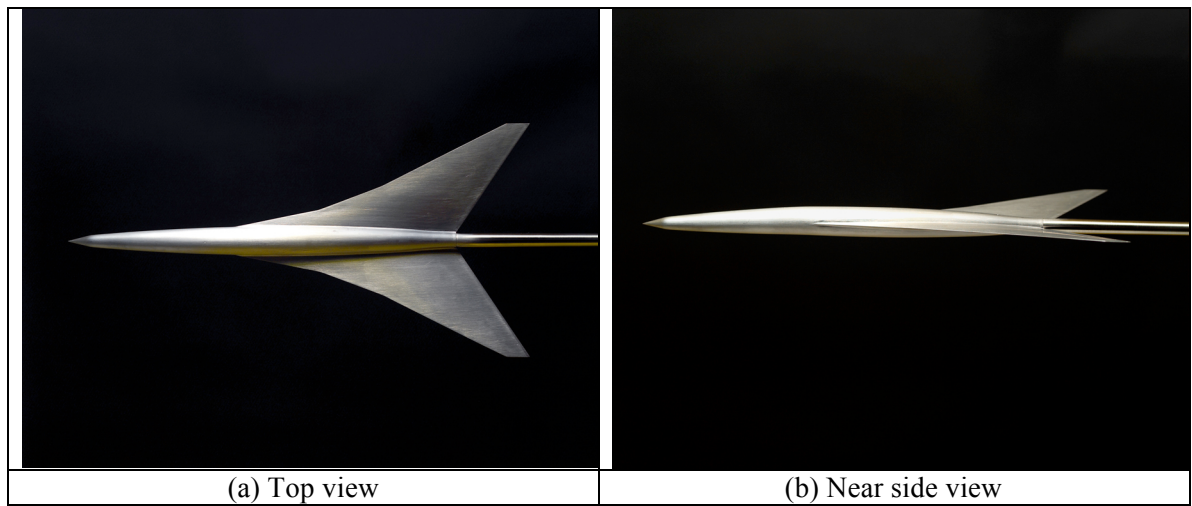
Figure 1: Straight-line segmented leading edge (SLSLE) model.
