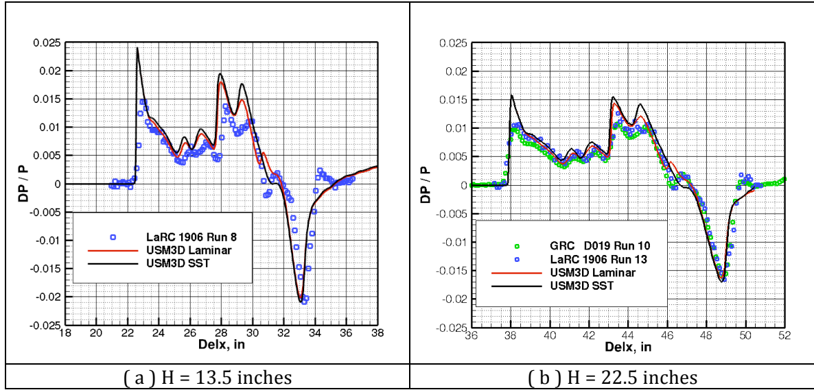
Figure 18: Centerline pressure signatures at various locations below model for M_\infty=2.0 , \alpha=2.3^\circ , Re_L=1.5 million. Comparison of USM3D laminar and SST turbulent solutions with wind tunnel data.
