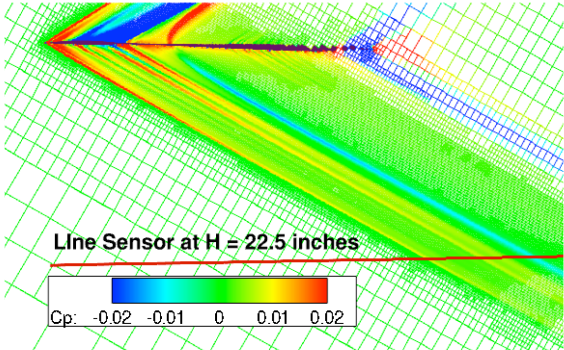
Figure 14: CART3D-AERO simulation of the SLSLE model. M_\infty=2.0 , \alpha=2.3^\circ , H=22.5 inches.
