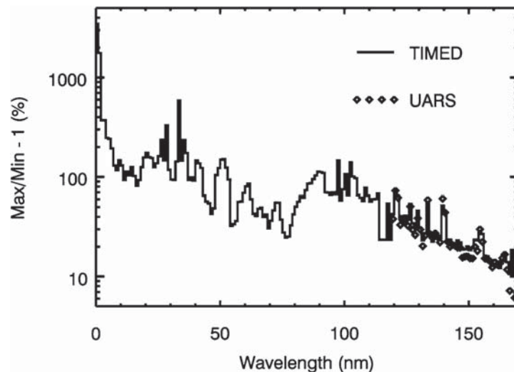
Figure 4 Solar EUV irradiance variations of the 11-year solar cycle. The TIMED/SEE results (line) agree very well with the UARS results (diamonds) in the far ultraviolet range (Woods et al. , 2005).
