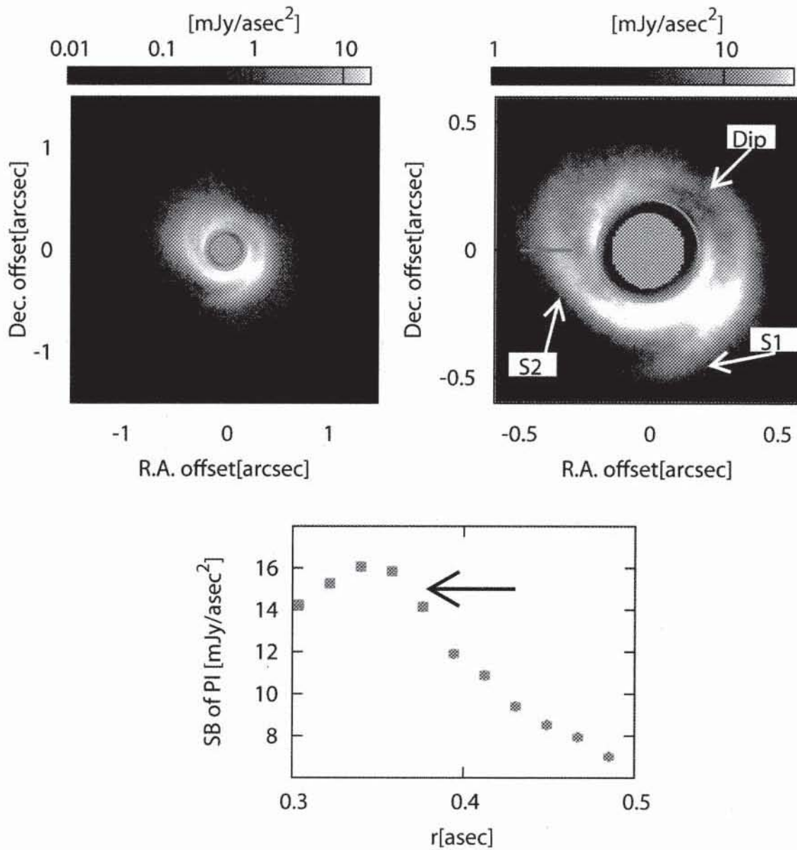
Fig. 2.— Top: PI image of SAO 206462 in the north-up configuration with log-stretch color scales. The filled orange circles at the center indicate the mask size ( r = 0''.15 ). The circles around have r = 0''.2 , exterior to which the features are considered to be real. The right panel is central region's closeup. Different color scales are used to enhance the spirals labeled as "S1" and "S2". The "Dip" may be due to depolarization. Bottom: PI profile along the red line in the top right panel. The arrow indicates the location of S2. The position errors are not shown for visibility.
