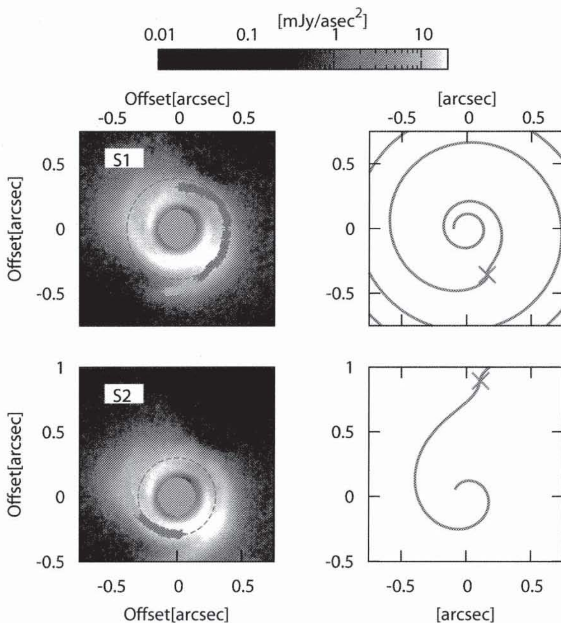
Fig. 4.— Left: Red and green points indicate the locations of the maxima of radial profiles for S1 (top) and S2 (bottom). The green ones are used for the fitting by Equation (1) (Section 4). Dashed lines indicate circles with r = 0''.39 (top) and r = 0''.3 (bottom). Right: The spiral shape given by Equation (1) with the best-fit parameters of S1 (top) and S2 (bottom). Crosses show the locations of (r_c, \theta_0) .
