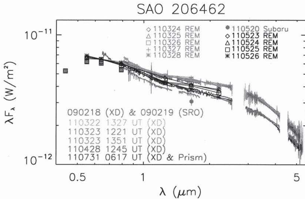
Fig. 1.— SED for SAO 206462 obtained by REM, adapted, in part, from Sitko et al. (2011). The REM observations consist of VRIJHK photometry. Also shown are spectra obtained with the SpeX spectrograph. See Section 2.3 for the data reduction techniques.
