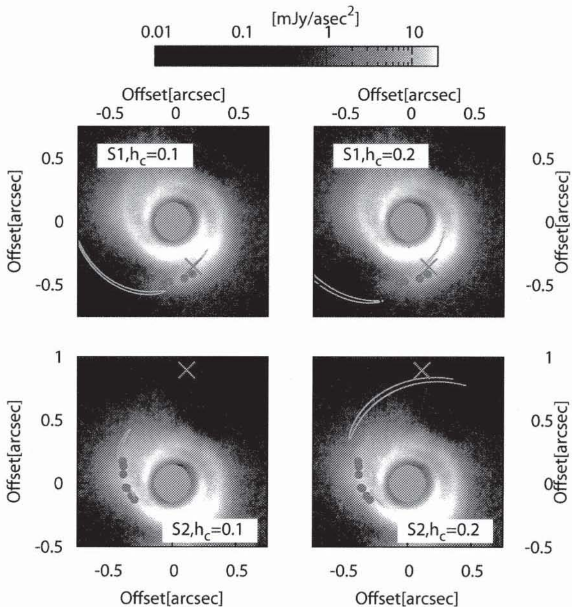
Fig. 5.— The parameter degeneracy of the fitting for S1 (top) and S2 (bottom) with h_c = 0.1 (left) and h_c = 0.2 (right). The red points show a part of the data fitted. The green curves indicate the 63.8% confidence level for the locations of (r_c, \theta_0) . The magenta crosses are (r_c, \theta_0) for the best-fit parameters. Note that the best-fit values of h_c are different from those shown in the figure.
