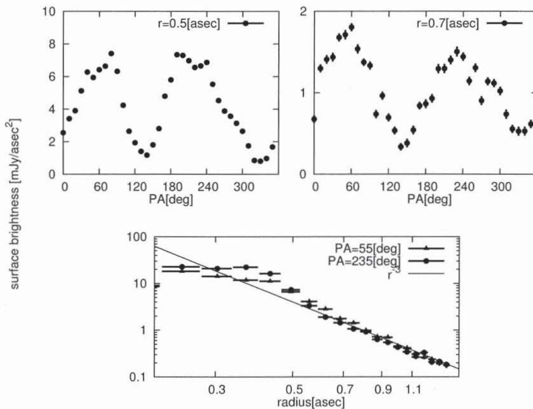
Fig. 3.— Top: Azimuthal SB profile at r = 0''.5 (left) and r = 0''.7 (right) with PA measured from north to east. Bottom: Radial profile along the major axis. Position errors indicate the FWHM of the PSF. SB errors are estimated using frame-by-frame deviations.
