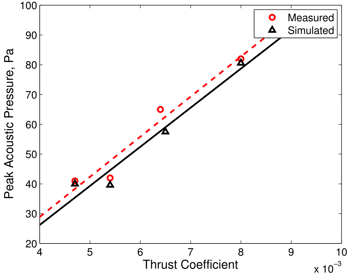
Figure 5.9: Measured and simulated variation in peak BVI acoustic pressure with thrust coefficient for the 45^\circ out-of-plane observer. Model uses parameters developed for the baseline case, C_T = 0.0047 and C_T = 0.0080 .
