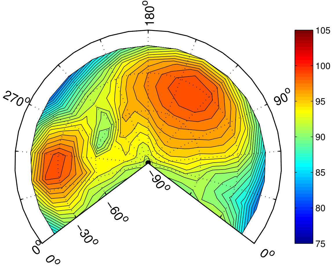
Figure B.3: Combined Bell 206 – OLS model BVISPL hemisphere estimate for Bell 206B3 -7.5^\circ flight path angle condition with advance ratio at 7500 ft.
