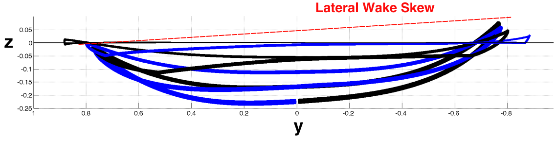
Figure 2.14: A head-on view of the Beddoes wake model.
