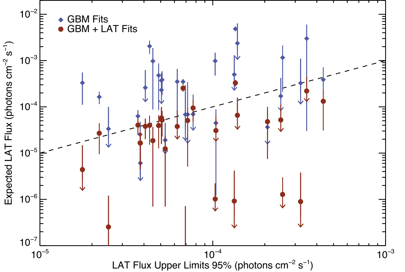
Fig. 5.— The expected photon flux, based on fits to the prompt GBM spectrum and duration plotted versus the LAT flux upper limit for each burst. When fitting only to the GBM data, roughly 50% of the bursts in the spectroscopic sample have expected LAT fluxes that exceed the LAT 95% CL flux upper limit. When fitting both the GBM and LAT data, only 23% of our sample have expected flux values that exceed the 95% CL LAT flux upper limit. The dashed line represents the line of equality.
