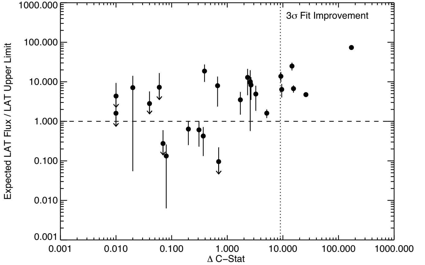
Fig. 9.— The ratio of the expected LAT flux (based on GBM-only fits) to the LAT 95% CL upper limit versus the \Delta C\text{-Stat} values for our spectroscopic subsample. The long and short dashed lines represents the line of equality between the LAT upper limits and the expected LAT flux and the \Delta C\text{-Stat} value representing a 3\sigma fit improvement respectively. The bursts for which a spectral break is statistically preferred have the most severe discrepancies between the GBM-only extrapolations and the LAT upper limits.
