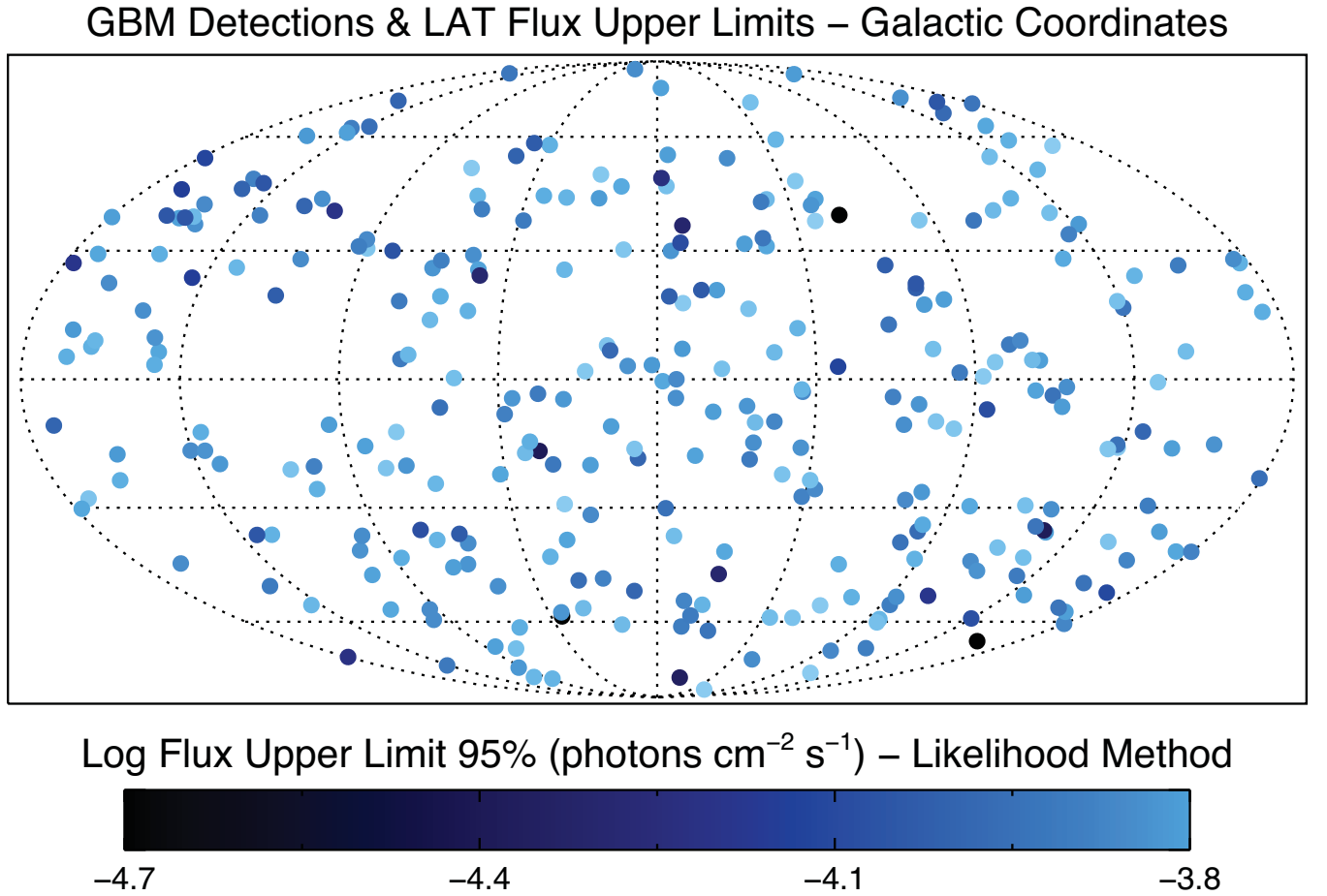
Fig. 4.— The celestial distribution of 288 gamma-ray bursts as detected by Fermi -GBM in the first 2.5 years of LAT operations that fell in the LAT FOV, plotted in Galactic coordinates. The colors represents the 95% CL LAT photon flux upper limits.
