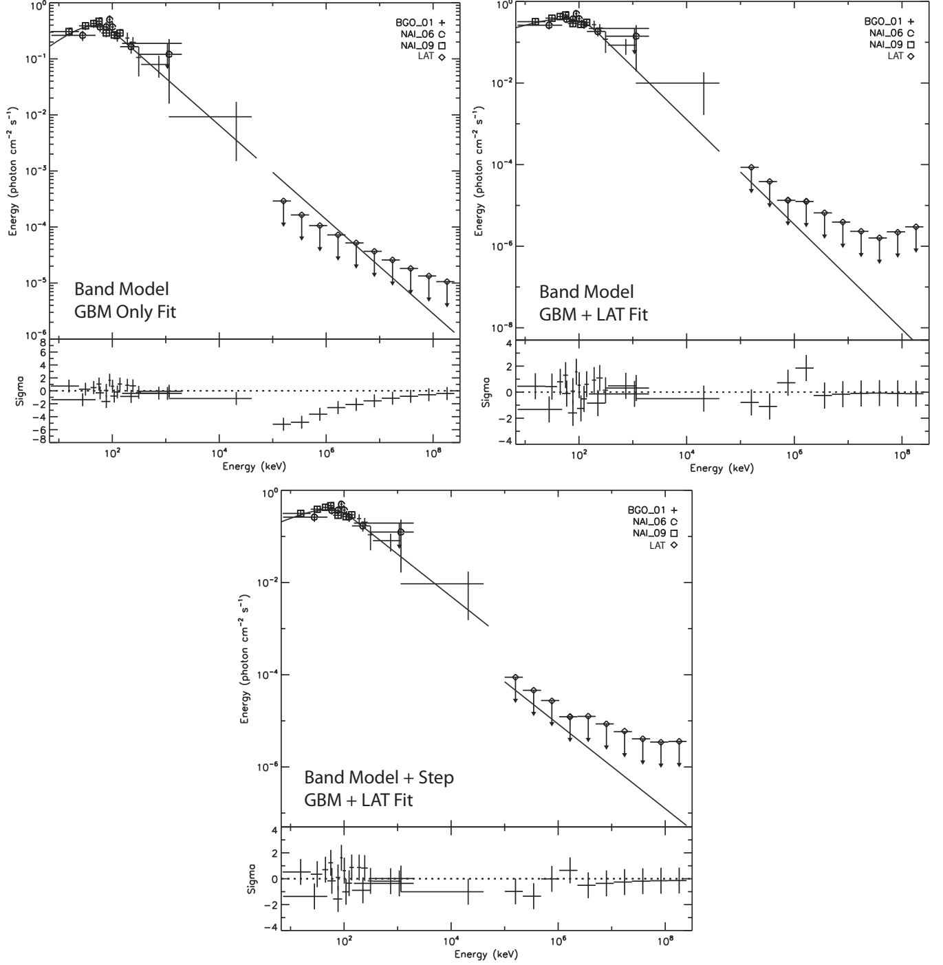
Fig. 8.— Example spectral fits showing (clockwise) a Band model fit to GBM data alone, a Band model fit to both the GBM and LAT data, and a Band model plus a step function fit to the GBM and LAT data.
