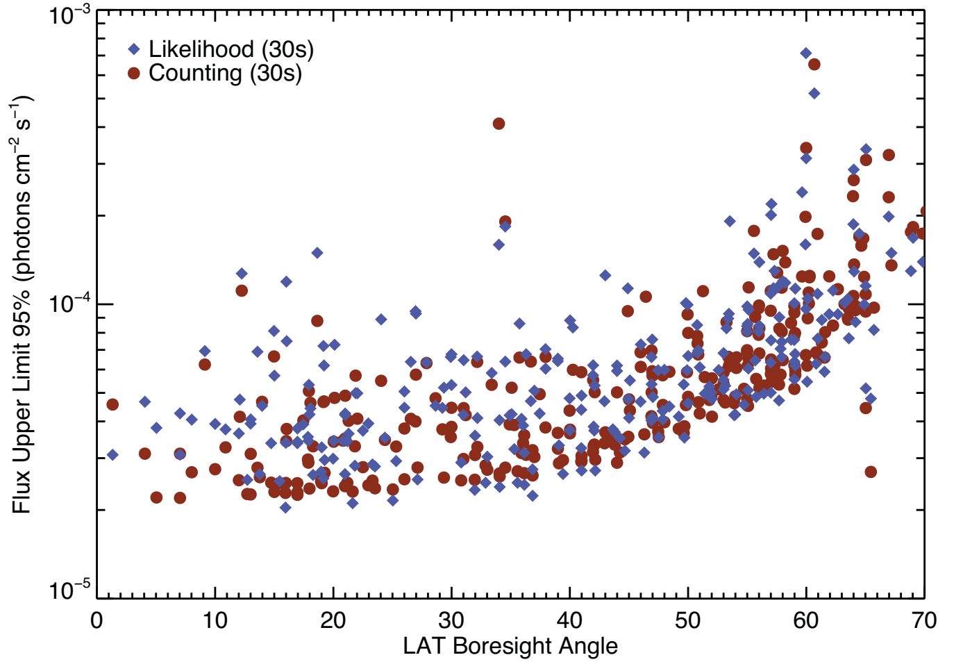
Fig. 3.— The 95% CL photon flux upper limits determined using the likelihood and counting methods as a function of off-axis angle. The decreasing exposure as a function of off-axis angle results in the shallowing of the LAT upper limits for bursts occurring away from the LAT bore sight.
