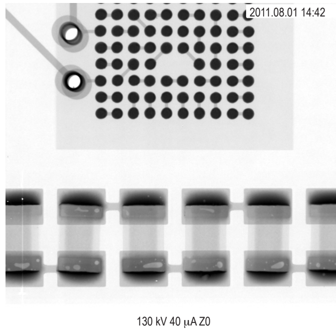
Figure 10. SnPb/SnPb solder postflight.
