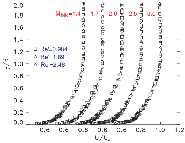
b) Normalized velocity profiles.
