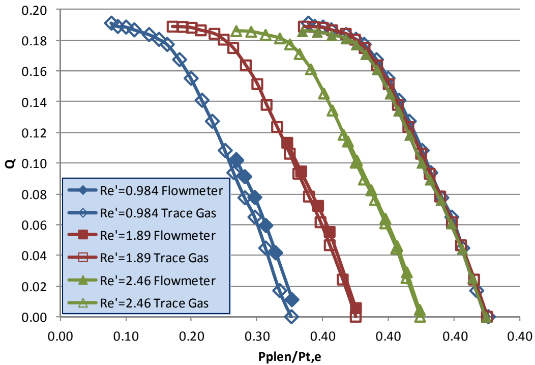
Figure 12.—Comparison of electronic flowmeter and trace gas system for CO1 at M_{b/k} = 1.4 .
