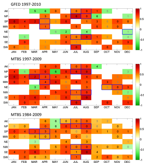
Fig. 7. Monthly cross correlation coefficients between PE and GFED BA (1997–2010, top) and MTBS BA (1997–2009, middle; 1984–2009, bottom). Numbers indicate the lead time between climate and BA in months. Black text signifies correlation coefficients with p < 0.05 , and grey text indicates correlation coefficients with 0.05 \leq p < 0.1 . Months with < 2\% of annual BA or months without statistically significant correlations between BA and climate variables ( p > 0.1 ) appear white. Blue boxes outline months with \geq 20\% of annual BA for each region.
