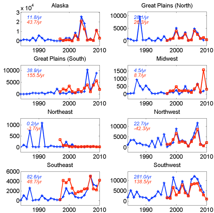
Fig. 4. Interannual variability in MTBS (blue) and GFED (red) BA for each NCA region. Values in each panel indicate the trends in annual BA ( \text{km}^2 \text{yr}^{-1} ) from robust linear regression for MTBS (1984–2009) and GFED (1997–2010) BA time series, as shown in Table 2.
