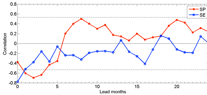
Fig. 9. Cross correlation coefficients between fire season BA and precipitation for the Southern Plains (SP) and Southeast (SE) regions for lead times of 0 to 24 months prior to the start of the fire season. Dashed lines indicate the limits for statistically significant correlation at the 95% confidence level.
