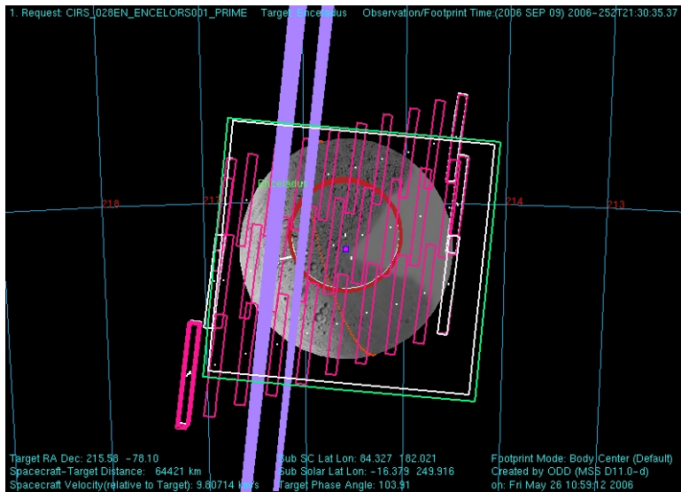
Figure 69: Enceladus Collaborative Observation taken in Rev 28. Includes ISS, UVIS, and VIMS pointing as well as CIRS FP1, FP3, and FP4.
