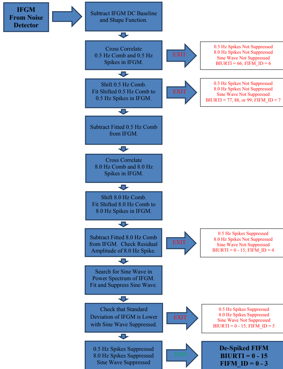
Figure 74: CIRS spike suppression algorithm block diagram
