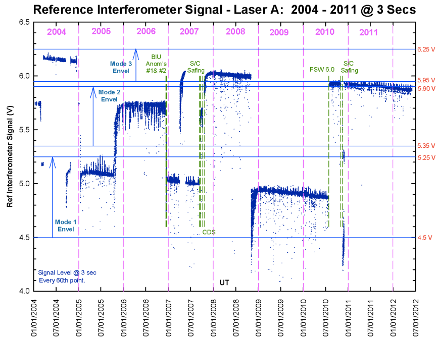
Figure 17: CIRS laser modes
