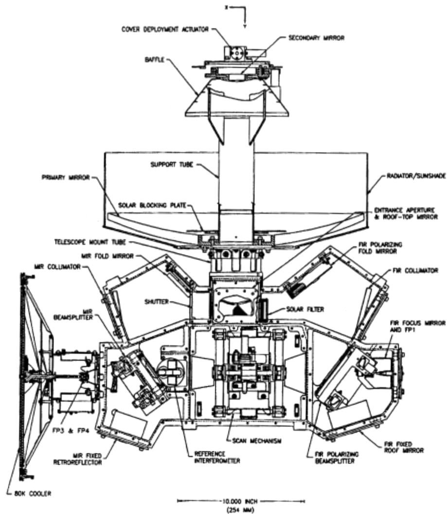
Figure 3: CIRS mechanical layout from Kunde et al. (1996).
