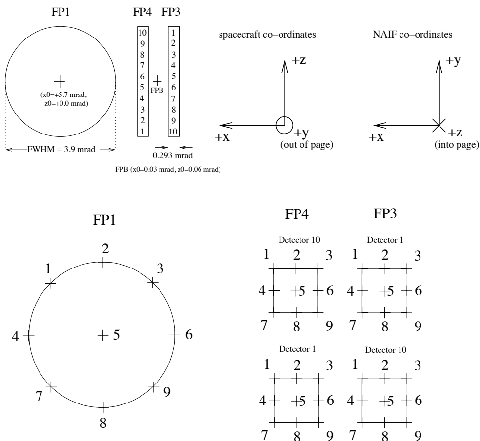
Figure 27: relative locations of CIRS detectors, showing numbering of pixels and q-points.
