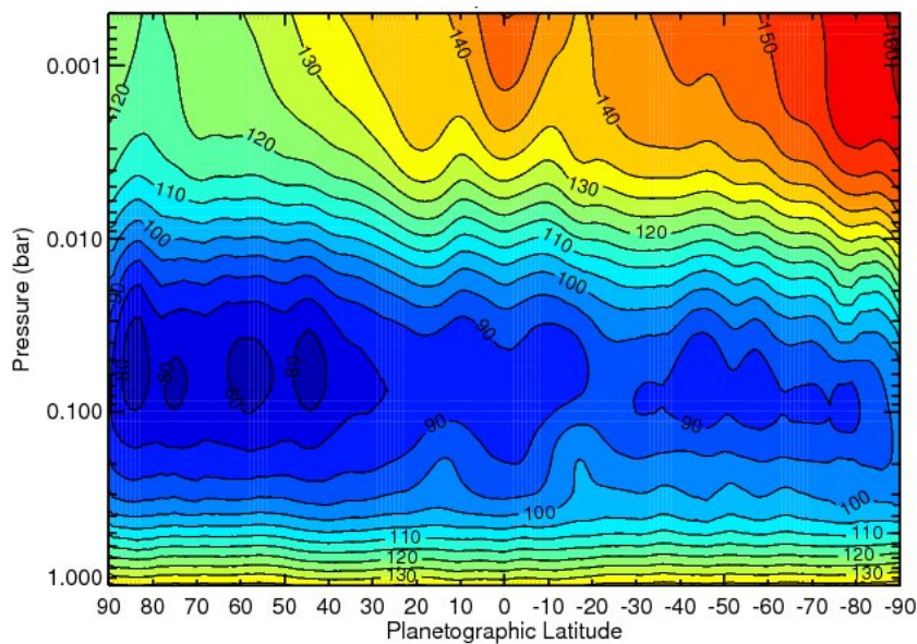
Figure 36: Saturn's temperature field derived from a co-addition of all available FIRMAP observations from the prime mission. The region between 10-80 mbar is a smooth interpolation between the two regions of CIRS sensitivity. Temperatures below 800 mbar are a smooth relaxation back to the a priori profile. See (Fletcher L. N., 2010) for details.
