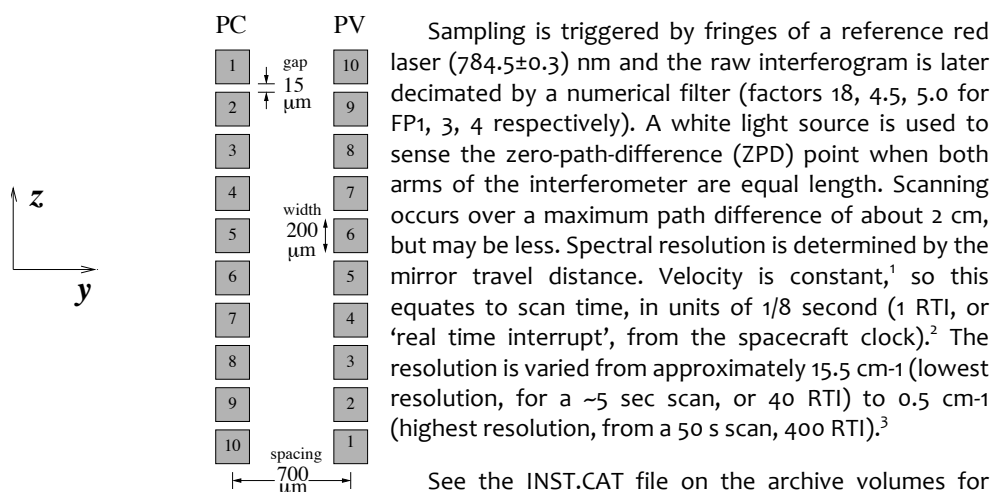
Figure 5: CIRS mid-infrared focal plane layout, showing detector spacing and numbering.
