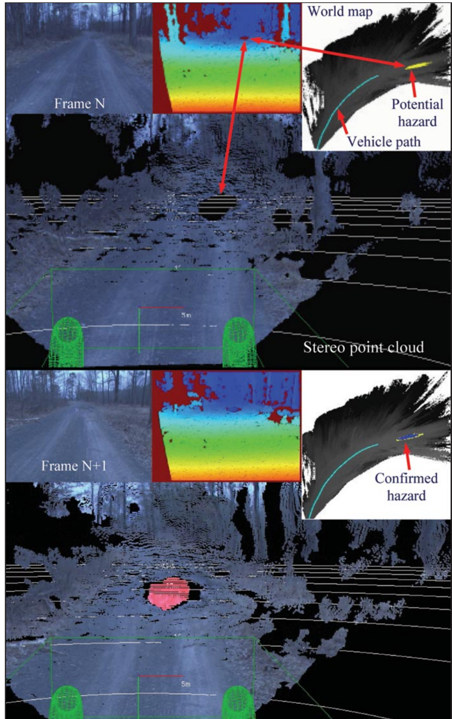
A hole in Stereo Range Data may be a water body still too small to be detected in image space. In this example, the hole was labeled a potential hazard in the world map in frame N. In the next frame, where there was previously a hole, there was range data that was detected as an object reflection, providing confirmation of a water body.
