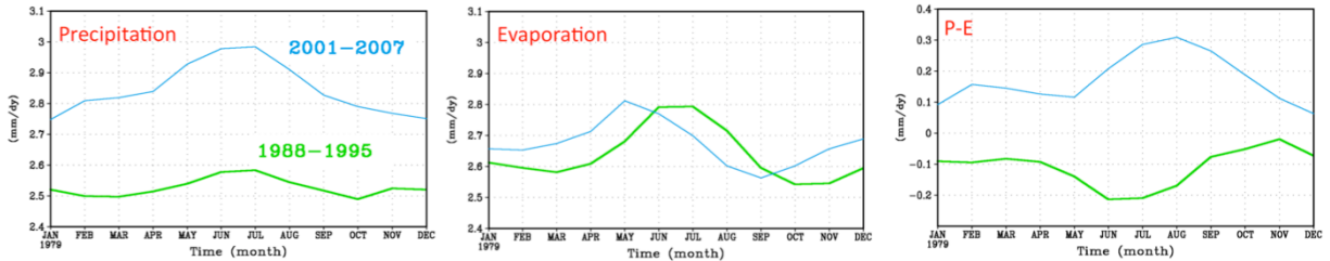
Figure 21: The annual cycle of the global mean precipitation, evaporation, and their difference, from MERRA. The pre-AMSU era is shown in green and the post-AMSU era in cyan.
