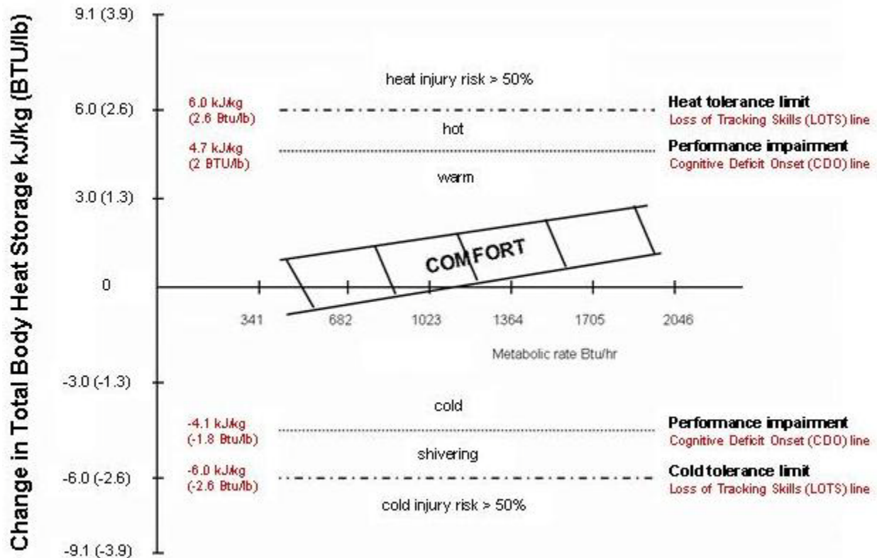
FIGURE E1-2 - HEAT STORAGE
