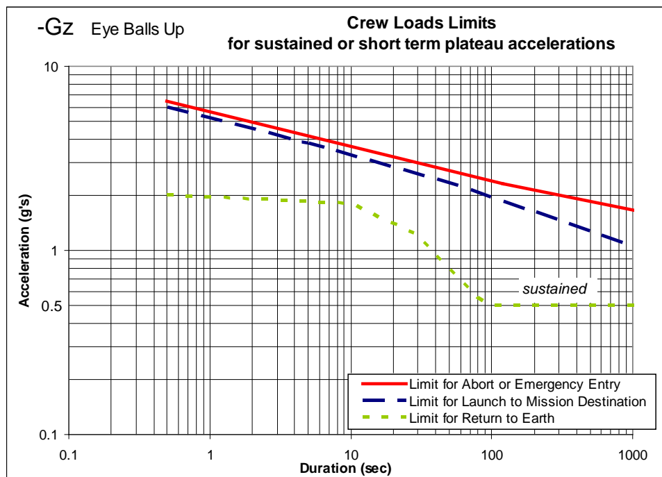
FIGURE 3.2.4.1.2-3 - - G_z LINEAR SUSTAINED ACCELERATION LIMITS
