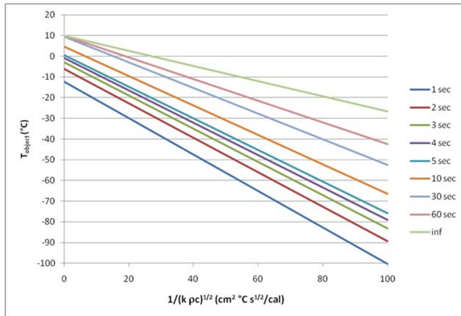
FIGURE 4.3.4.2-1 - ALLOWABLE COLD TOUCH TEMPERATURE DURATION
