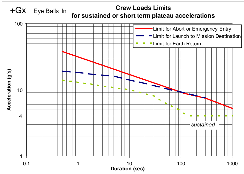
FIGURE 3.2.4.1.2-1 - + G x LINEAR SUSTAINED ACCELERATION LIMITS
