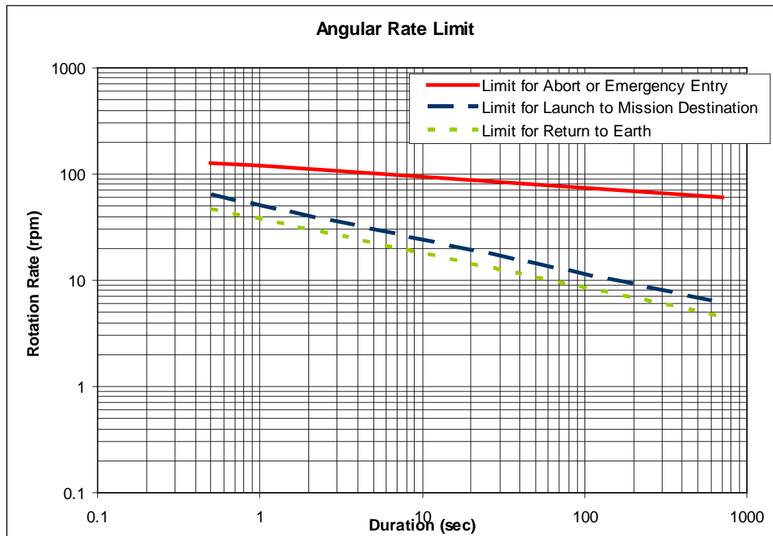
FIGURE 3.2.4.4.3-1 - ANGULAR RATE LIMITS
