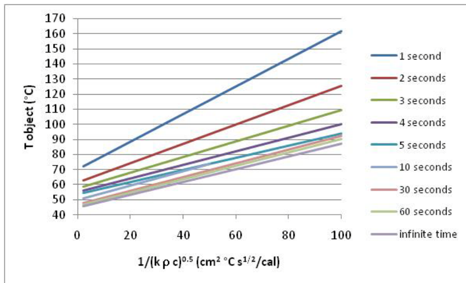
FIGURE 4.3.4.1-1 - ALLOWABLE HOT TOUCH TEMPERATURE DURATION
