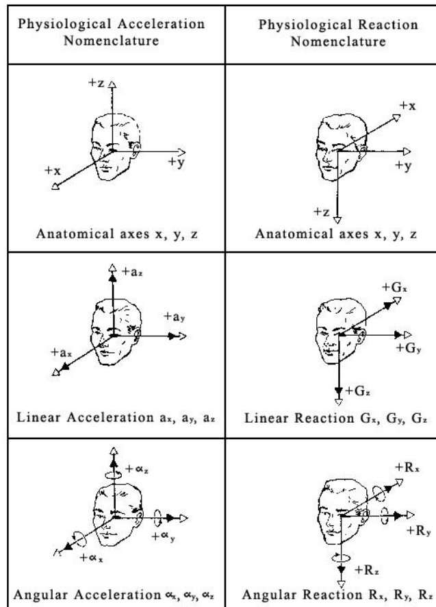
FIGURE C2-1 - ACCELERATION ENVIRONMENT COORDINATE SYSTEM
