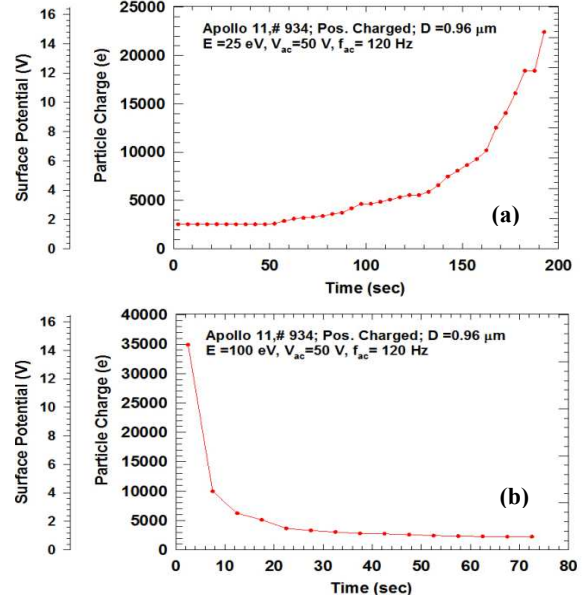
Fig.4. A positively charged 0.96 \mu\text{m} Apollo 11 dust grain at V_{ac} =50V, f_{ac} =120Hz a) Charges with 25eV electron beam b) Discharges with 100 eV electron
