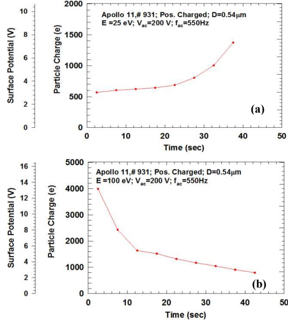
Fig.2. A positively charged 0.54 \mu\text{m} Apollo 11 dust grain at V_{ac} =200V, f_{ac} =550Hz a) Charges with 25eV electron beam and b) Discharges with 100 eV elec-
