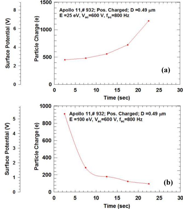
Fig.3. A positively charged 0.49 \mu\text{m} Apollo 11 dust grain at V_{ac} =600V, f_{ac} =800Hz a) Charges with 25eV electron beam and b) Discharges with 100 eV
