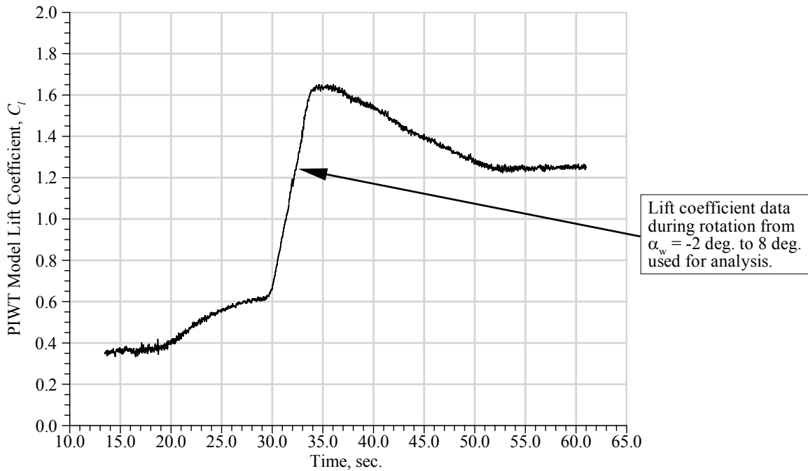
Figure 8.—Sample lift coefficient versus time profile for the simulated takeoff acceleration and wing rotation used in the PIWT tests.
