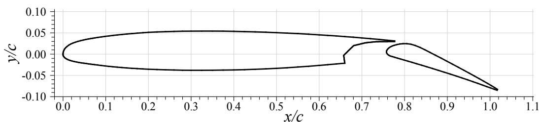
Figure 7.—Thin, high-performance airfoil section used in the PIWT testing, reference chord = 6.0 ft (1.8 m).
