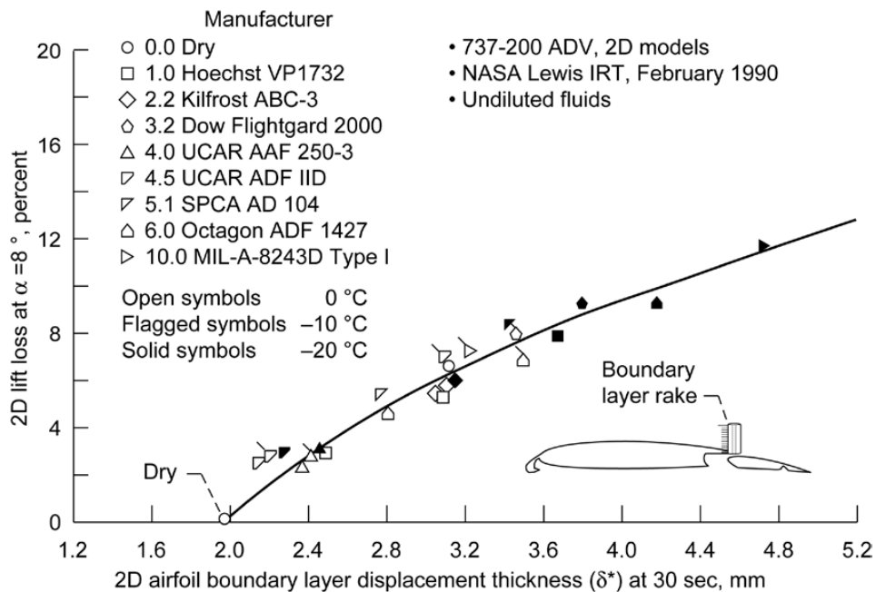
Figure 1.—Correlation between percent lift loss and boundary-layer displacement thickness as measured on the 2-D model at \alpha_w = 8^\circ for various fluids at air temperatures of 0, -10 and -20 °C, after Hill and Zierden (Ref. 14).
