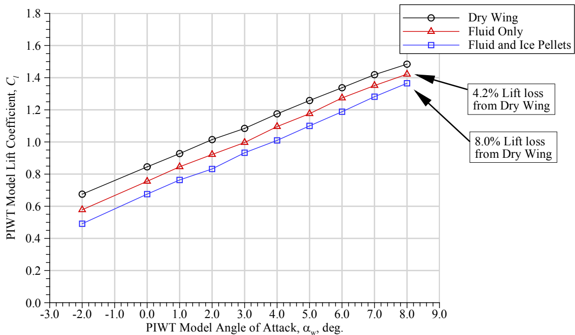
Figure 9.—Sample lift coefficient versus angle of attack data for three configurations—dry wing, uncontaminated fluid only and fluid with ice-pellet contamination.
