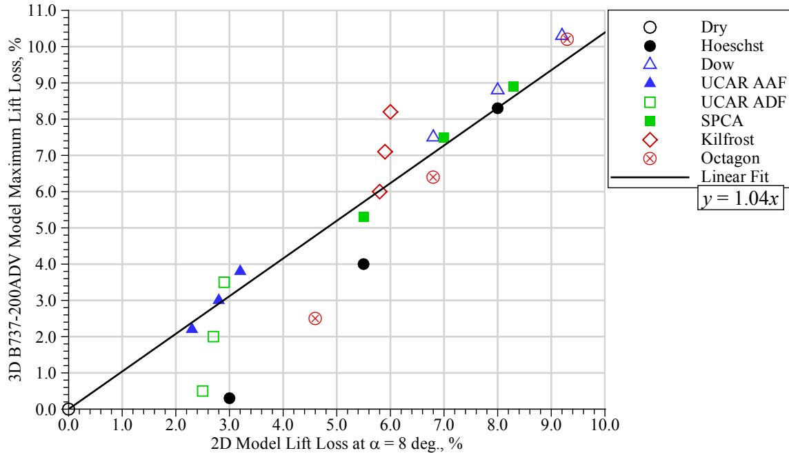
Figure 3.—Correlation between percent lift loss on the 2–D model at \alpha_w = 8^\circ and percent maximum lift loss on the 3–D B737-200ADV model for a given fluid at a given temperature in the Phase II IRT tests. Note that there are three data points for each fluid representing 0, -10 and -20 °C. Data extracted from Hill (Ref. 15).
