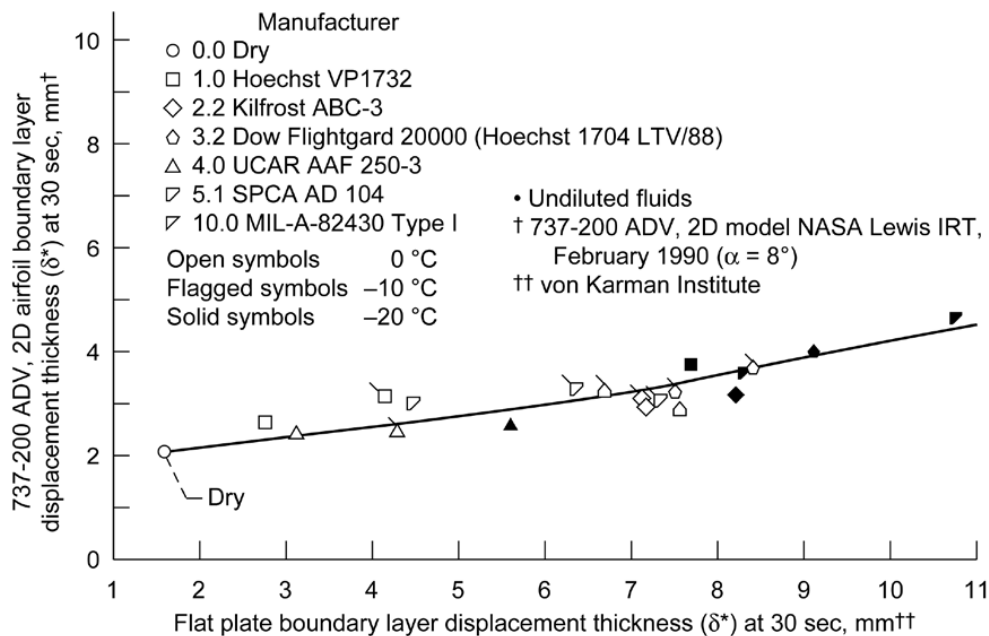
Figure 4.—Correlation between displacement thickness measured on the 2-D B737-200ADV wing section in the IRT and the displacement thickness measured on the flat plate in the von Kármán Institute experiment, after Hill and Zierten (Ref. 14).
