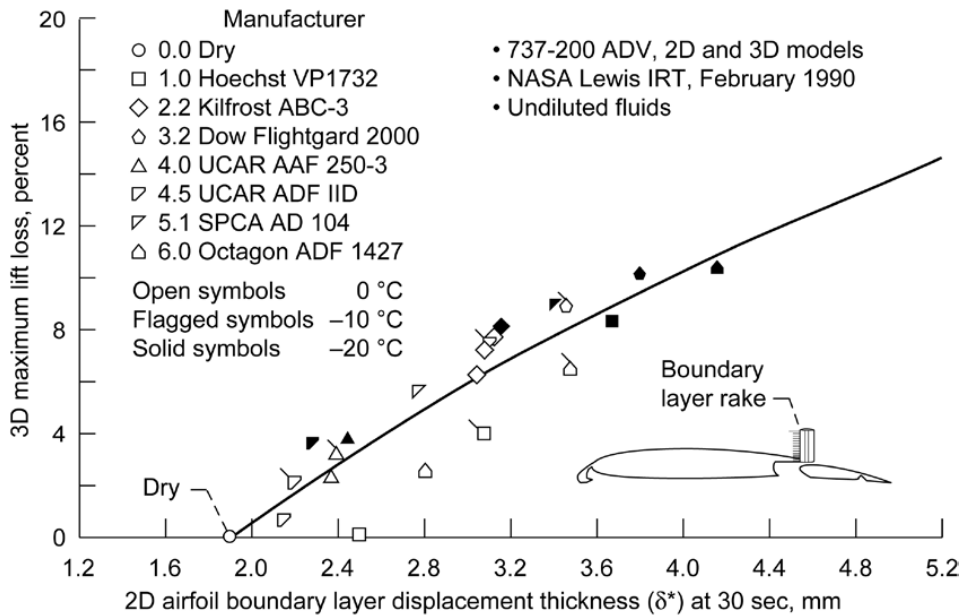
Figure 2.—Correlation between 3–D B737-200ADV model percent maximum lift loss and 2–D model boundary-layer displacement thickness at \alpha_w = 8^\circ for various fluids at air temperatures of 0, –10 and –20 °C, after Hill and Zierten (Ref. 14).
