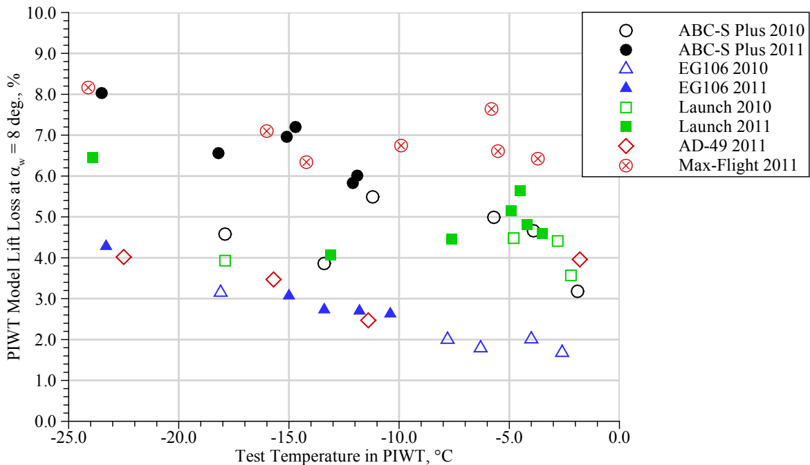
Figure 10.—Summary of uncontaminated fluid tests for PIWT test campaigns in 2010 and 2011.
