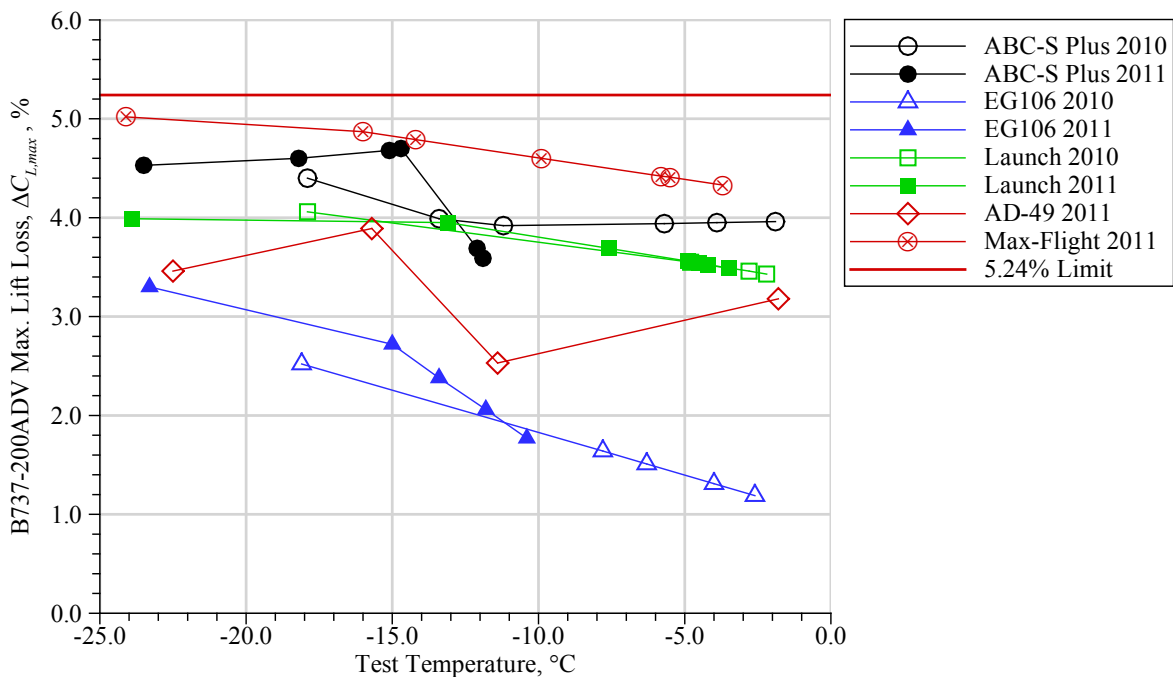
Figure 13.—B737-200ADV maximum lift loss for the PIWT test temperatures calculated using AAT data shown in Figure 12 using Equation (1).
