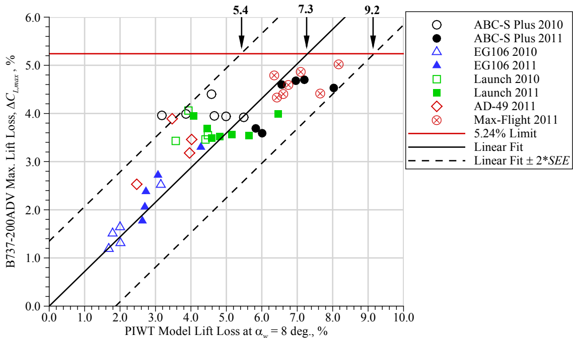
Figure 14.—Correlation between percent lift loss on the PIWT model at \alpha_w = 8^\circ and percent maximum lift loss on the 3–D B737-200ADV airplane for the uncontaminated fluid tests.
