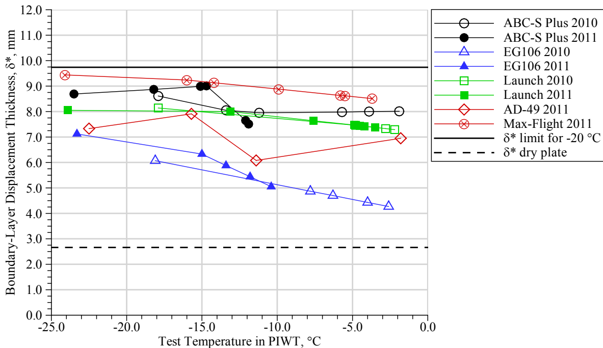
Figure 12.—Boundary-layer displacement thickness values associated with PIWT test temperatures.
