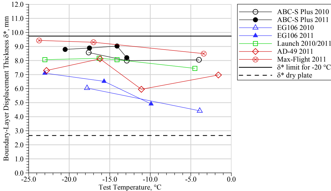
Figure 11.—Summary of AMIL AAT results for fluid samples used in the 2010 and 2011 PIWT test campaigns.
