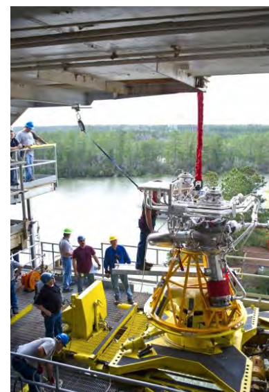
Engineers and technicians install the J-2X powerpack into the Stennis Space Center (SSC) A-1 test stand
