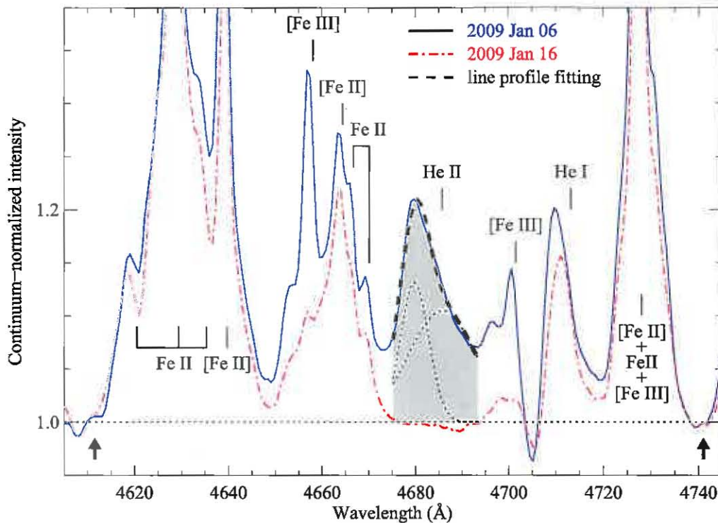
Figure 2. He II \lambda 4686 at minimum (dash-dotted red line) and maximum (solid blue line). The observed line profile was fitted by two gaussian components (dotted lines) and the result (dashed line) was used to measure the radial velocity. The two arrows indicate the regions adopted as continuum level for the He II \lambda 4686 emission line. The equivalent width was derived by direct integration under the line profile (gray shaded area).
