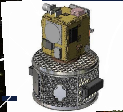
Ride Share Adapter (Space Access Technology)
