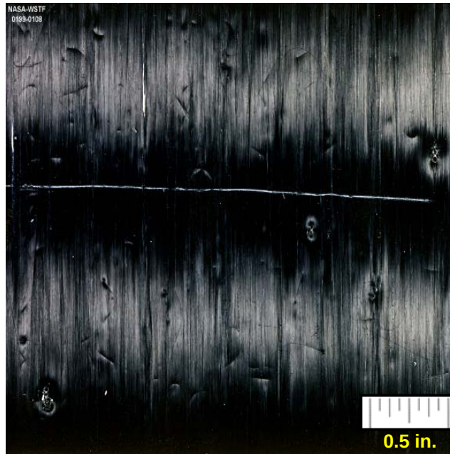
Figure A-3 Level I Scratch/Scuff/Abrasion (Cut)
