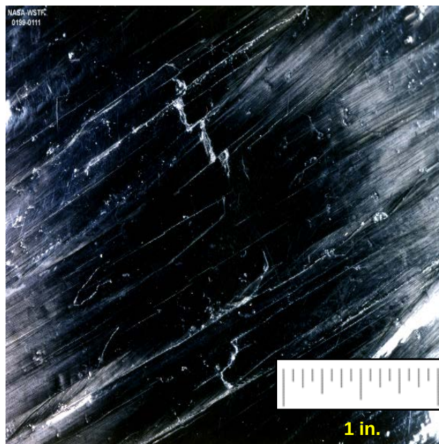
Figure A-6 Level II Impact/Mechanical Damage (Broken Tows)
