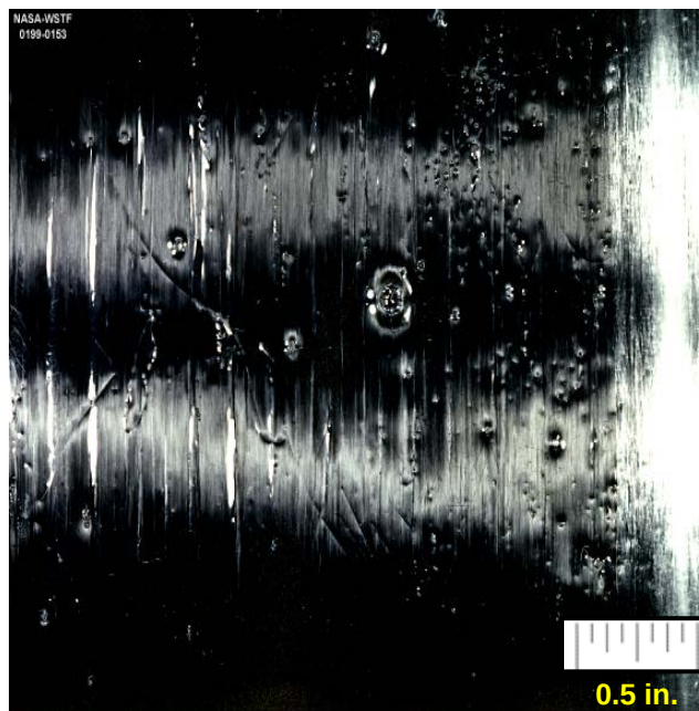
Figure A-2 Level I Manufacturing (Matrix Indications)
