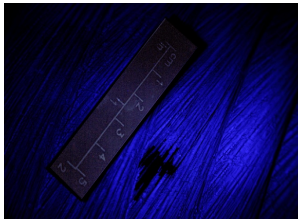
Figure A-8 Level II Impact/Mechanical Damage (Specialized Coating Black Light Illumination)
