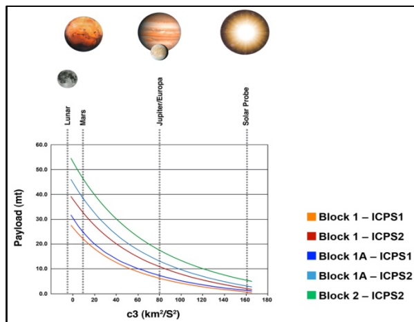
Figure 4. SLS C3 Capabilities.
