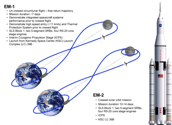
Figure 1. Initial SLS/Orion Exploration Missions.
