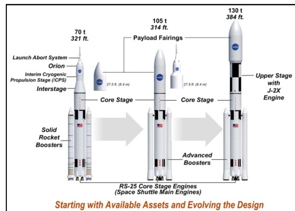
Figure 2. SLS Block 1 (70 t), Block 1A (105 t), and Block 2 (130 t).
