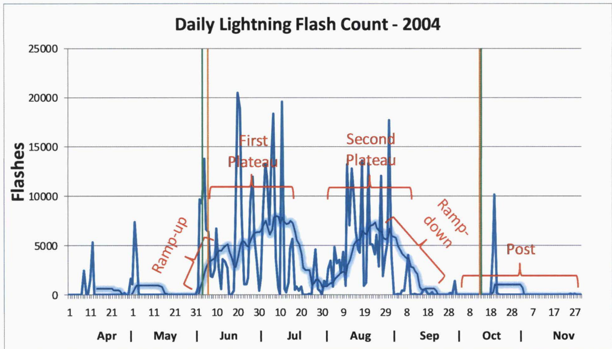
Figure 7. As in Figure 6, but for 2004.
