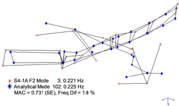
[G] S4-1A F2 Mode 3 vs. Analytical Mode 102
