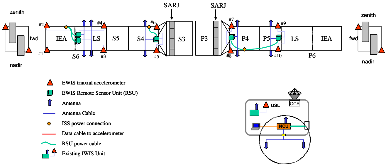
Figure 4-1. EWIS Architecture
