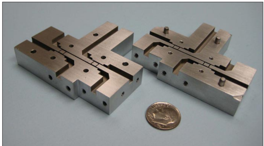
This photo of the fabricated Serial Combiner shows the split-block construction arrangement.
