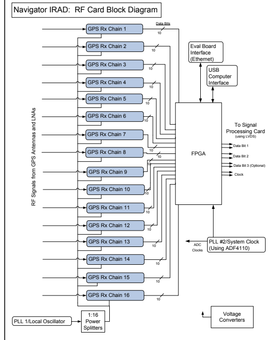
Figure 5: Block diagram of array front-end design.
