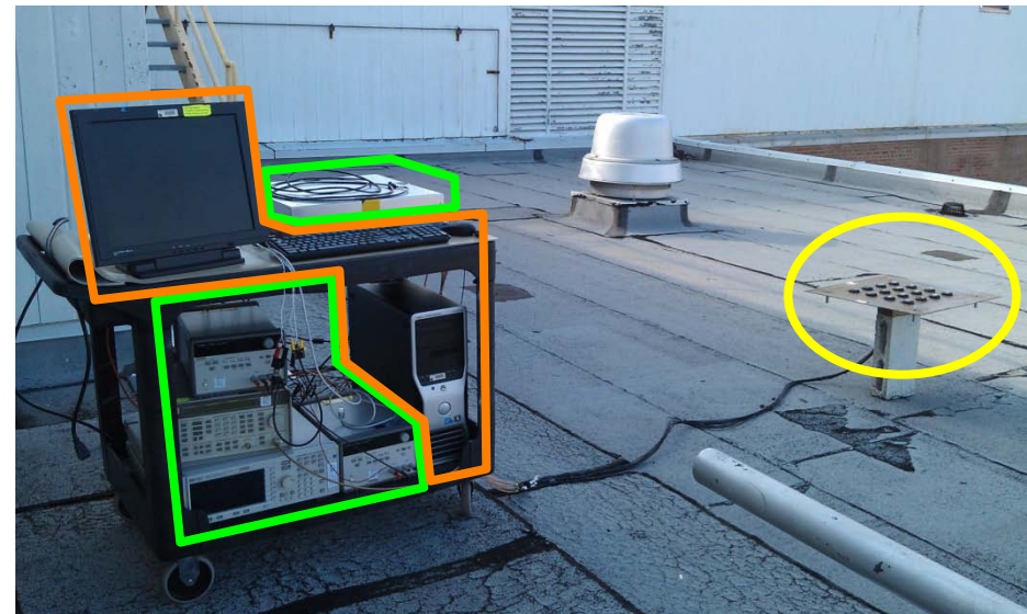
Navigator GPS receiver with antenna array
