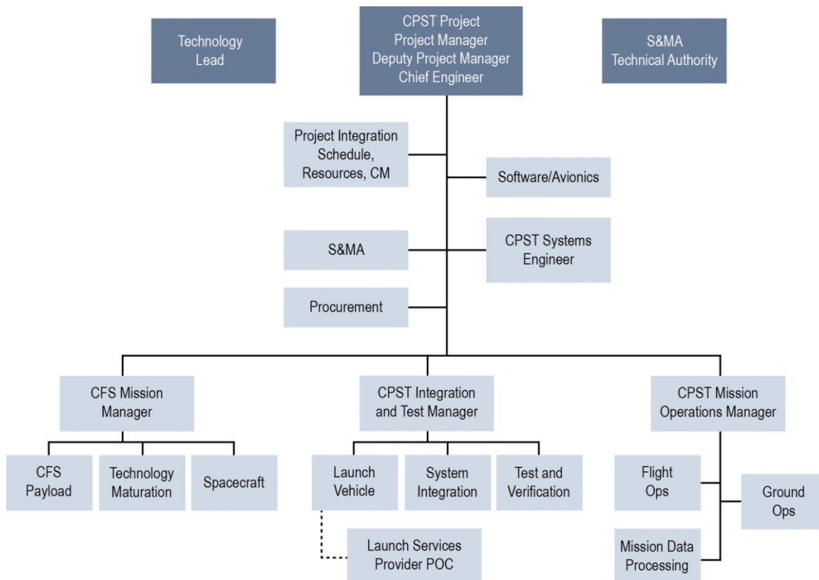
Fig. 1: Project Organization
