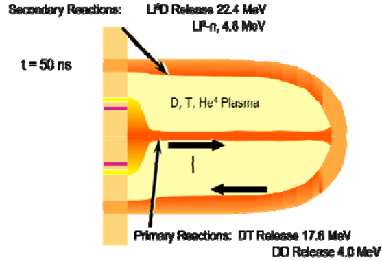
Figure 3 – Li 6 liner provides anode return path
