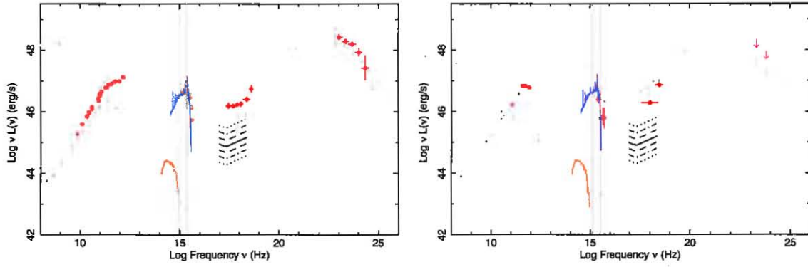
Fig. 7. The SEDs of 4C 38.41 ( z = 1.814 ; left ) and 1Jy 0537-286 ( z = 3.104 ; right ). Simultaneous data are shown in red; non-simultaneous literature or archival data are shown in light gray. Note that the UVOT data of these medium and high redshift objects matches quite well the QSO template of Vandenberg et al. (2001) that we use to estimate the thermal emission from the blue bump ( blue line ). The emission from the host galaxy ( orange line ) is very low compared to other components. The observed X-ray emission from these sources is more than 3\sigma above the expected emission from accretion derived from Eq. 2. In both cases, the optical light is dominated by radiation from the accretion while the X-rays originate from the non-thermal component.
