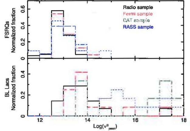
Fig. 17. The rest-frame synchrotron \nu_{\text{peak}}^S distributions of FSRQs and BL Lacs in different samples. Black solid histograms: radio sample; red dashed histograms: Fermi -LAT sample; green dot-dashed histograms: Swift BAT sample; blue dotted histograms: RASS sample.
