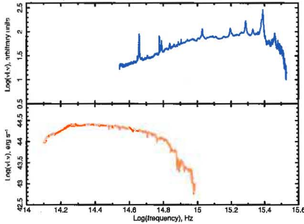
Fig. 4. Top panel: The SDSS template of Vanden Berk et al. 2001 for the broad-line and thermal emission from a QSO. Bottom panel: The giant elliptical galaxy template of Mannucci et al. 2001. See text for details.
