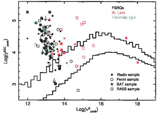
Fig. 20. \log(\gamma_{\text{peak}}^{\text{SSC}}) , obtained from Eq. 3 for all the objects in our samples for which we could obtain \nu_{\text{peak}}^S and \nu_{\text{peak}}^{\text{IC}} is plotted against \log(\nu_{\text{peak}}^S) in the rest-frame of the blazars. The two black lines delimit the area predicted by simple homogeneous SSC models obtained through extensive Monte Carlo simulations (see Abdo et al. 2010a, for details).
