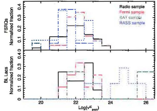
Fig. 18. The rest-frame inverse Compton \nu_{\text{peak}}^{\text{IC}} distributions of FSRQs and BL Lacs in different samples. Black solid histograms: radio sample; red dashed histograms: Fermi -LAT sample; green dot-dashed histograms: Swift BAT sample; blue dotted histograms: RASS sample.
