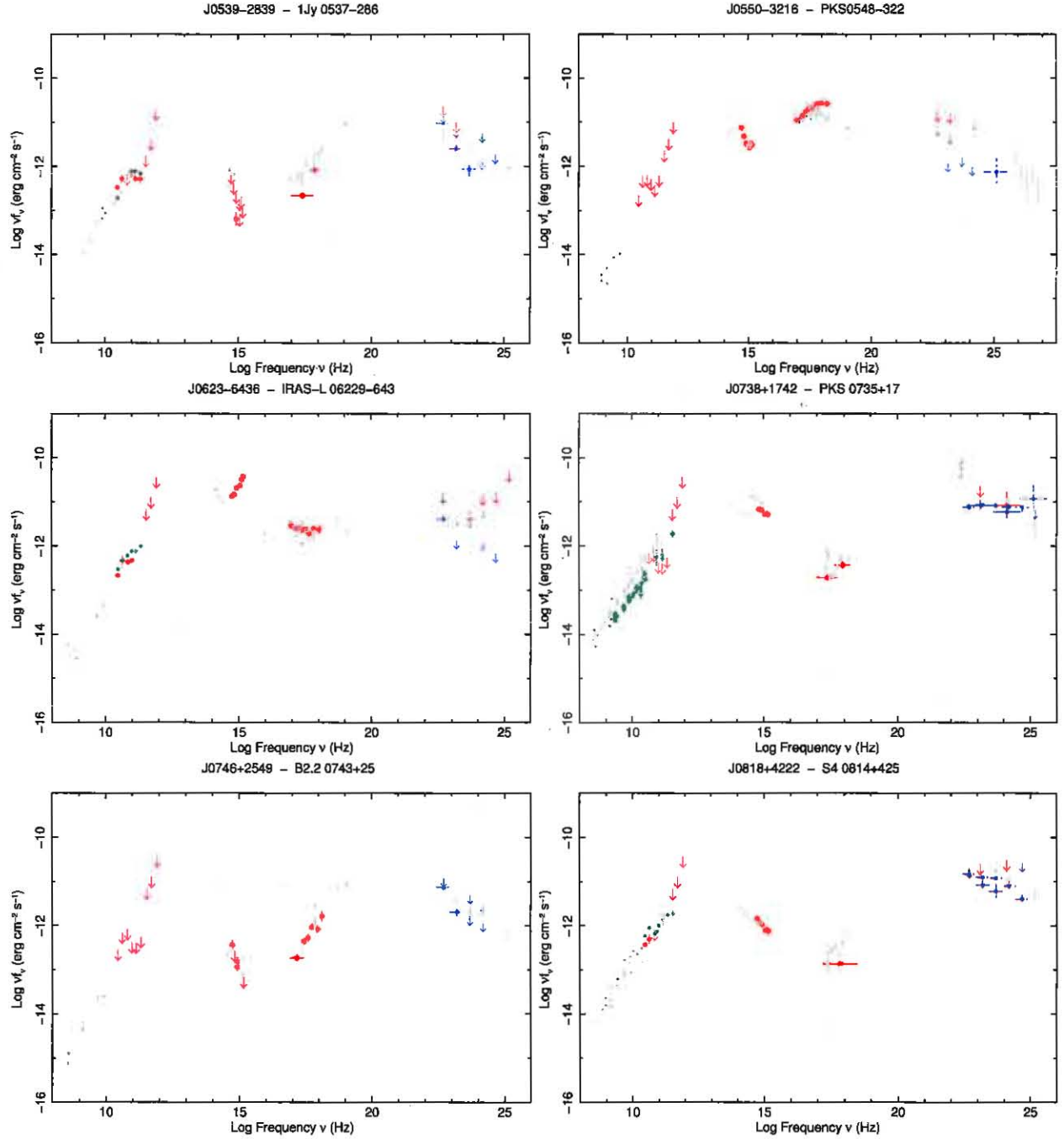
Fig. 28. The SED of 1Jy 0537–286 (J0539–2839, top left), PKS 0548–322 (J0550–3216, top right), IRAS-L 06229–643 (J0623–6436, middle left), PKS 0735+17 (J0738+1742, middle right), B2.2 0743+25 (J0746+2549, bottom left), and S4 0814+425 (J0818+4222, bottom right). Simultaneous data are shown in red; quasi-simultaneous data, i.e. Fermi data integrated over 2 months, Planck ERCSC and non-simultaneous ground based observations are shown in green; Fermi data integrated over 27 months are shown in blue; literature or archival data are shown in light gray.
