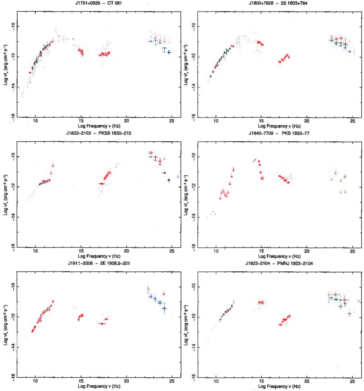
Fig. 37. The SED of OT 081 (J1751+0939, top left), S5 1803+784 (J1800+782, top right), PKS B 1830-210 (J1833-2103, middle left), PKS 1833-77 (J1840-7709, middle right), 2E 1908.2-201 (J1911-2006, bottom left), and PMNJ 1923-2104 (J1923-2104, bottom right). Simultaneous data are shown in red; quasi-simultaneous data, i.e. Fermi data integrated over 2 months, Planck ERCSC and non-simultaneous ground based observations are shown in green; Fermi data integrated over 27 months are shown in blue; literature or archival data are shown in light gray.
