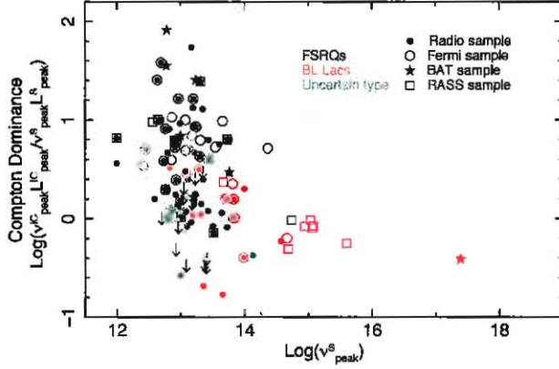
Fig. 21. The logarithm of the Compton dominance is plotted as a function of \log(v^S_{\text{peak}}) for all sources for which v^S_{\text{peak}} and v^C_{\text{peak}} could be reliably determined.
