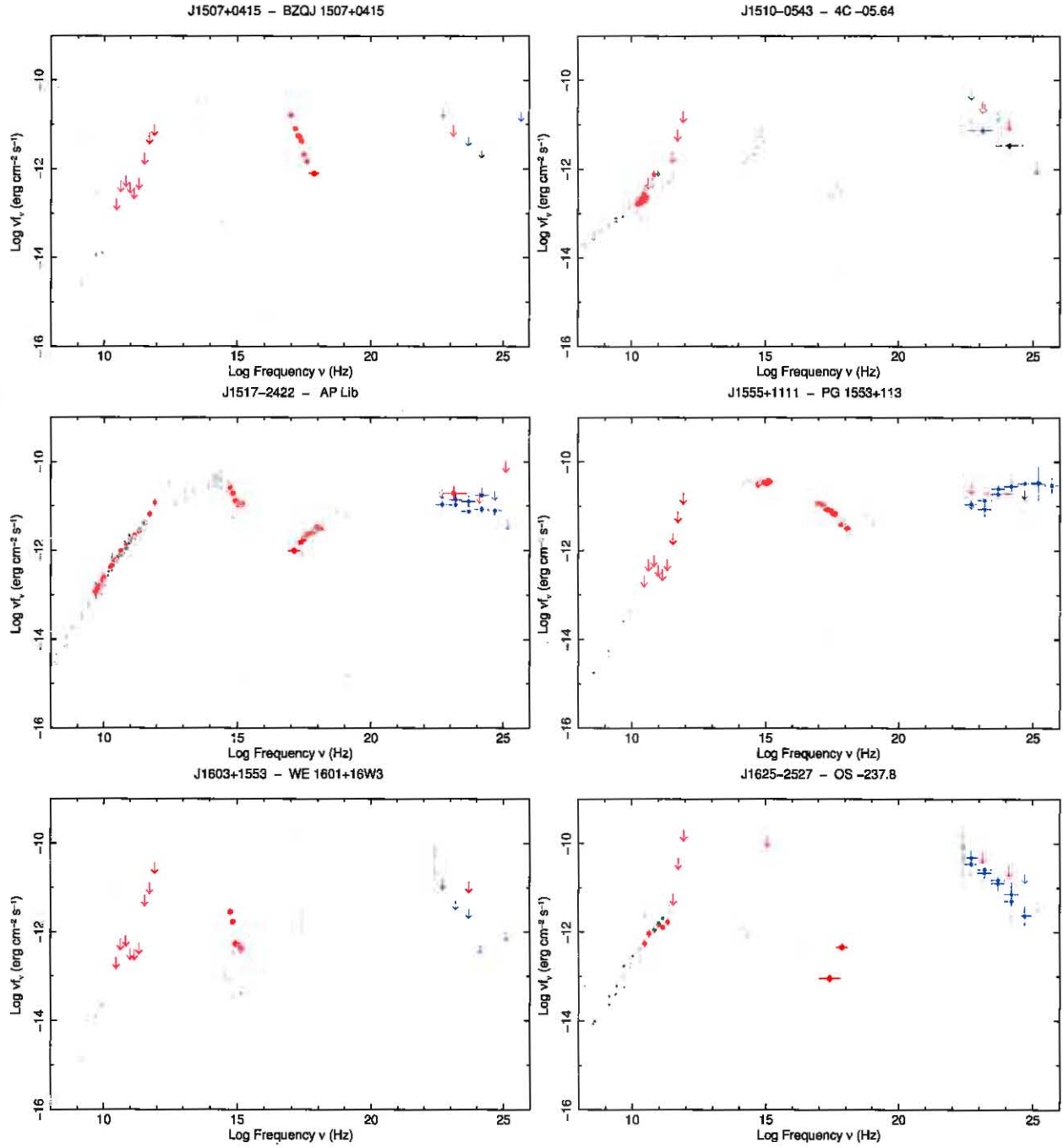
Fig. 35. The SED of BZQJ 1507+0415 (J1507+0415, top left), 4C-05.64 (J1510-0543, top right), AP Lib (J1517-2422, middle left), PG 1553+113 (J1555+1111, middle right), WE 1601+16W3 (J1603+1553, bottom left), and OS -237.8 (J1625-2527, bottom right). Simultaneous data are shown in red; quasi-simultaneous data, i.e. Fermi data integrated over 2 months, Planck ERCSC and non-simultaneous ground based observations are shown in green; Fermi data integrated over 27 months are shown in blue; literature or archival data are shown in light gray.
