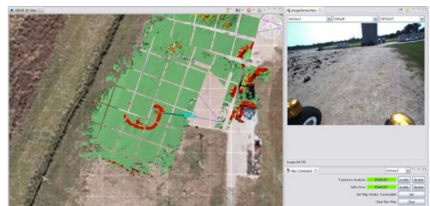
Figure 15: Map of rock field (top) and E-Stop operator walking in front of rover (red trail) causing the robot to stop.
