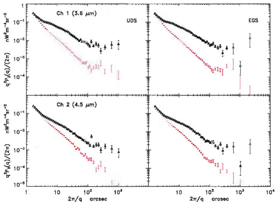
Fig. 2.— Fluctuations from the (A + B) (black triangles) and \frac{1}{2}(A - B) maps (red error bars).
