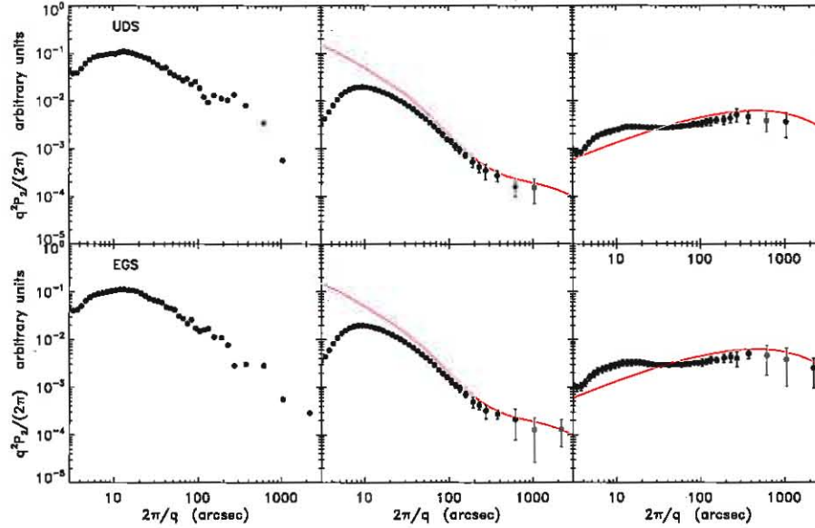
Fig. A-13.— Masking effects on fluctuations with different power spectra. The results are based on 100 realizations of CIB with a given power spectrum and field parameters. Filled dots show the mean of the realizations and error bars correspond to one standard deviation. Left: Power spectrum of the mask. Middle: Ordinary galaxies with the spatial power spectrum from Sullivan et al. (2007). The input template without the mask convolution is shown with a red line. Right: high- z \Lambda CDM. The input template without the mask convolution is shown with a red line. (The convolution with the instrument beam is omitted in all cases.)
