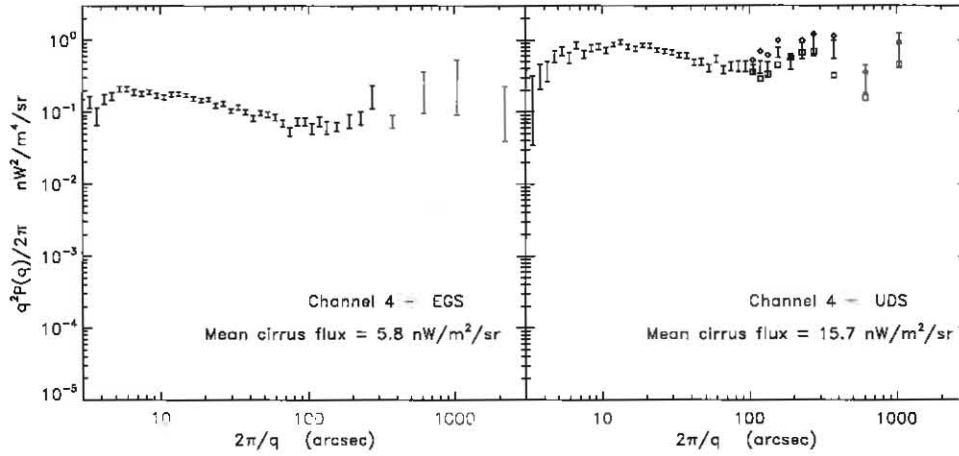
Fig. 7.— Source subtracted CIB fluctuations at 8\ \mu\text{m} for EGS and UDS fields. In the UDS field at 8\ \mu\text{m} the maps contain a notable large-scale artifact which translates into a diagonal stripe in Fourier space. To probe the sensitivity of the resultant power spectrum to this feature we have computed the power spectrum independently from the two quadrants in the Fourier space: (q_x < 0, q_y > 0) (containing the stripe feature) and (q_x > 0, q_y > 0) . The power spectra from these are shown with open diamonds and squares respectively and can be seen to be within the statistical uncertainties of the overall spectrum.
