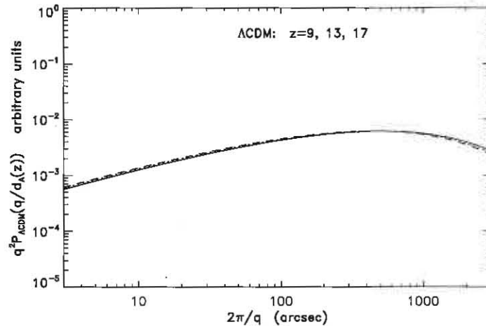
Fig. A-12.— High- z shape of the concordance \Lambda CDM power spectrum projected to z = 9, 13, 17 .
