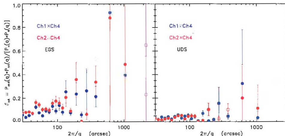
Fig. 8.— Coherence, C_{n4} \equiv \frac{P_{n4}(q) * P_{n4}(q)}{P_n(q) P_4(q)} , for 1-4 (blue) and 2-4 (red) for EGS (left) and UDS (right) fields. Open symbols correspond to scales where P_{n4} < 0 . The relative statistical uncertainties on the coherence resulting from cosmic variance are given by \sqrt{12/N_q} which is shown with the error bars; this is valid at small C when all the power spectra can be assumed independent. With N_q plotted in Fig. 1 this uncertainty is of order 100% for the last three points in the EGS field.
