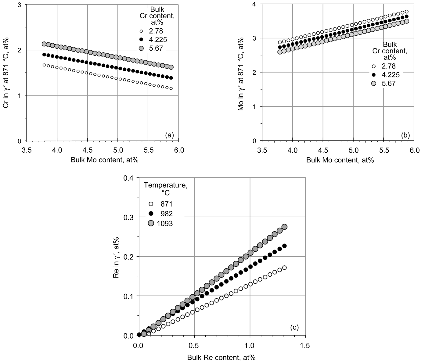
Figure 19.—Regression model output curves for the estimated \gamma' phase chemistry. (a) Cr concentration in the \gamma' phase at 871 °C as a function of bulk Mo content and 2.78, 4.225, and 5.67 at% Cr, with Re fixed at its midrange level. (b) Mo concentration in the \gamma' phase at 871 °C as a function of the bulk Mo content and 2.78, 4.225, and 5.67 at% Cr. (c) Re concentration in the \gamma' phase as a function of bulk Re content at 871, 982, and 1093 °C.
