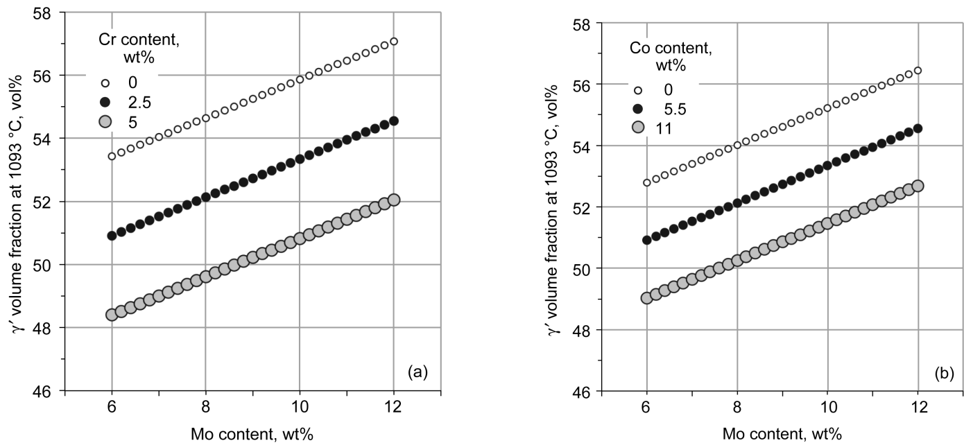
Figure 8.—Regression model output curves for estimated \gamma' volume fraction at 1093 °C as a function of bulk Mo content. (a) 0, 2.5, and 5.0 wt% Cr, with Co and Re fixed at their midrange levels (5.5 wt% and 2 wt%, respectively). (b) 0, 5.5, and 11 wt% Co, with Cr and Re fixed at their midrange levels.
