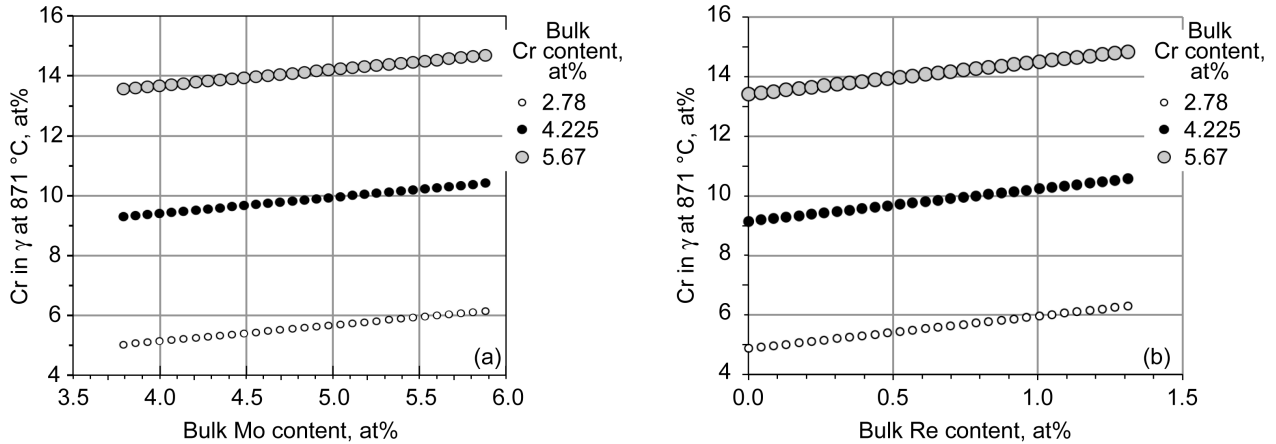
Figure 16.—Regression model output curves for the estimated Cr concentration in the g phase at 871 °C. (a) As a function of the bulk Mo content at 2.78, 4.225, and 5.67 at% Cr with Re fixed at its midrange level. (b) As a function of the bulk Re content at 2.78, 4.225, and 5.67 at% Cr with Mo fixed at its midrange level.
