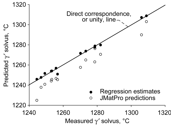
Figure 3.—Predicted versus measured \gamma' solvus is shown for regression estimates determined in this study and for JMatPro 6.0 predictions.
