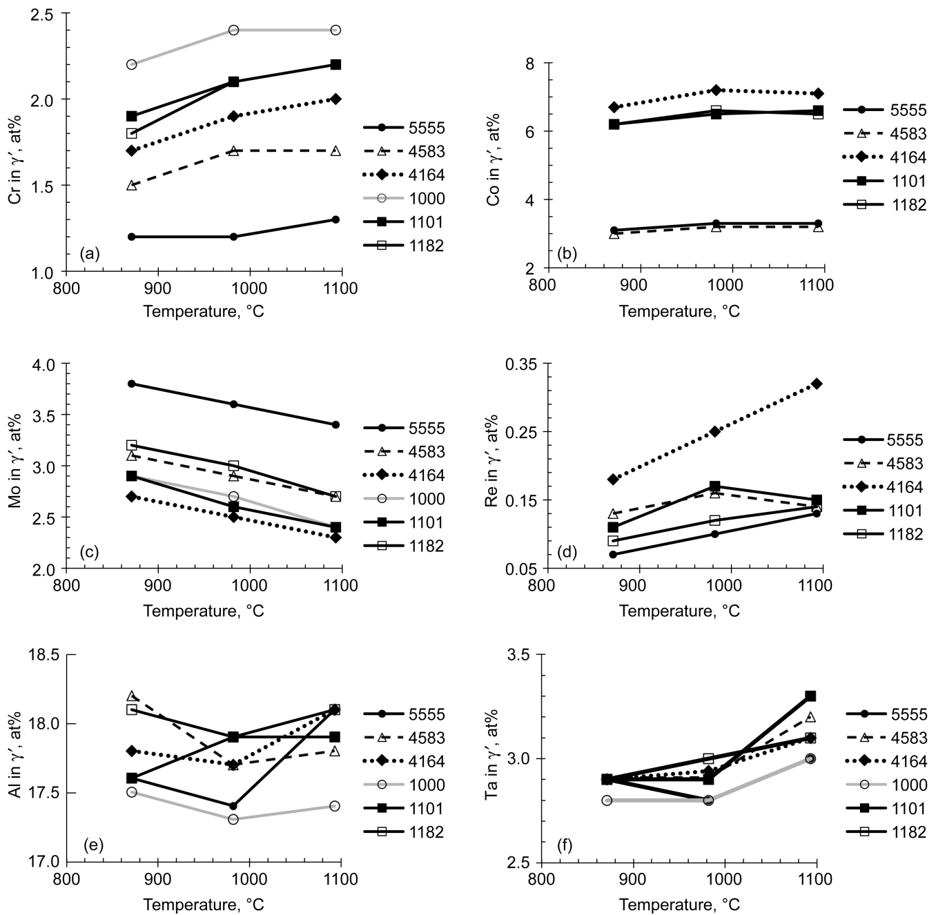
Figure 15.—Concentrations of elements in the \gamma' phase are shown as a function of temperature for a subset of LDS alloys. (a) Cr. (b) Co. (c) Mo. (d) Re. (e) Al. (f) Ta.
