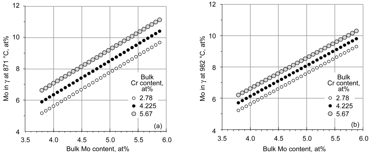
Figure 17.—Regression model output curves for the estimated Mo concentration in the g phase as a function of the bulk Mo content at 2.78, 4.225, and 5.67 at% Cr. (a) At 871 °C. (b) At 982 °C.
