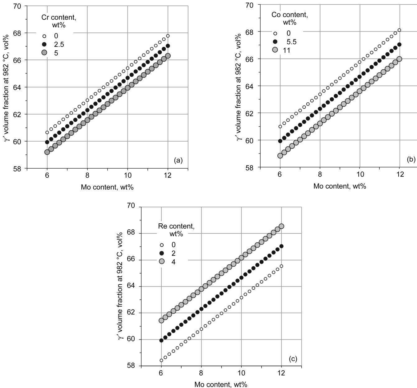
Figure 7.—Regression model output curves for estimated \gamma' volume fraction at 982 °C as a function of bulk Mo content. (a) 0, 2.5, and 5.0 wt% Cr, with Co and Re fixed at their midrange levels (5.5 and 2 wt%, respectively). (b) 0, 5.5, and 11 wt% Co, with Cr and Re fixed at their midrange levels. (c) 0, 2, and 4 wt% Re, with Cr and Co fixed at their midrange levels.
