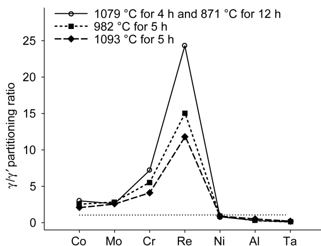
Figure 13.—g/g' partitioning ratio for each major alloying element in LDS-1101 as a function of aging temperature. The fine dotted line represents a partitioning ratio of 1.0. A partitioning ratio greater than 1.0 indicates that the element partitions to the g matrix, and a partitioning ratio less than 1.0 indicates that the element partitions to the g' phase.
