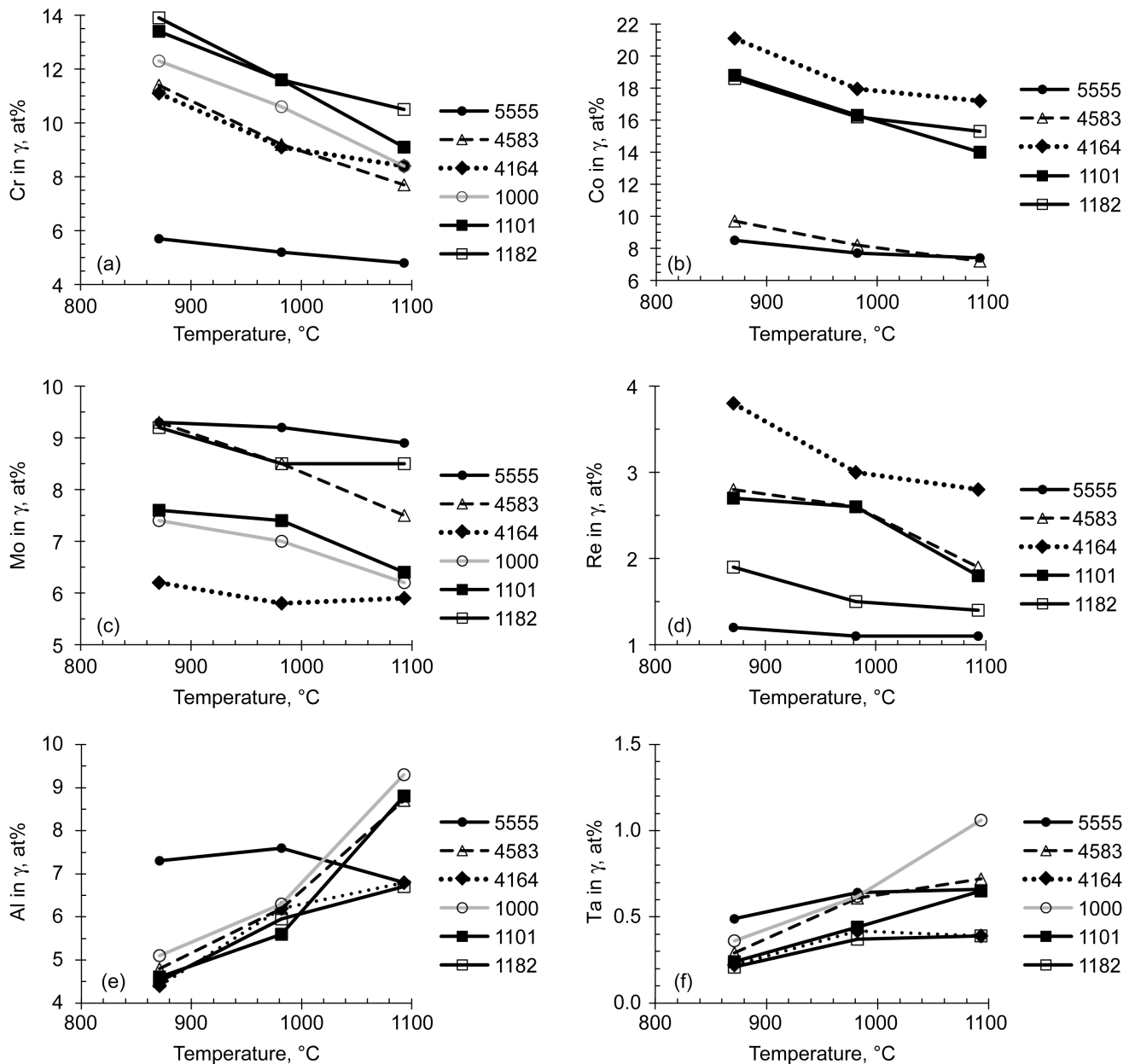
Figure 14.—Concentrations of elements in the g matrix are shown as a function of temperature for a subset of LDS alloys. (a) Cr. (b) Co. (c) Mo. (d) Re. (e) Al. (f) Ta.
