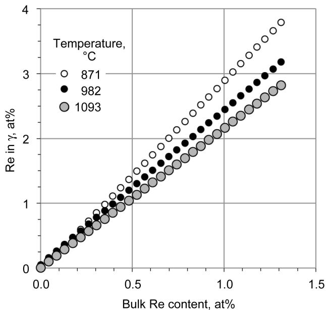
Figure 18.—Regression model output curves for the estimated Re content in the \gamma phase as a function of the bulk Re content at 871, 982, and 1093 °C.
