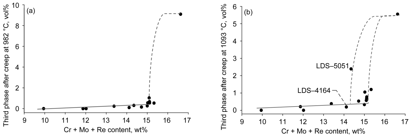
Figure 12.—Third phase volume fraction after creep testing as a function of analyzed Cr + Mo + Re levels (wt%) in the bulk. (a) At 982 °C. (b) At 1093 °C.
