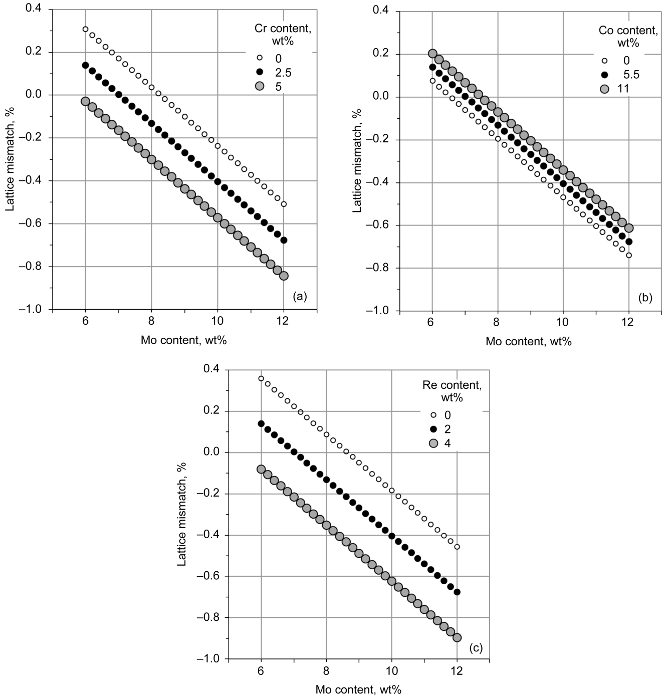
Figure 24.—Regression model output curves for estimated g-g lattice mismatch at room temperature as a function of bulk Mo content. (a) 0, 2.5, and 5 wt% Cr, with Co and Re fixed at their midrange levels. (b) 0, 5.5, and 11 wt% Co, with Cr and Re fixed at their midrange levels. (c) 0, 2, and 4 wt% Re, with Cr and Co fixed at their midrange levels.
