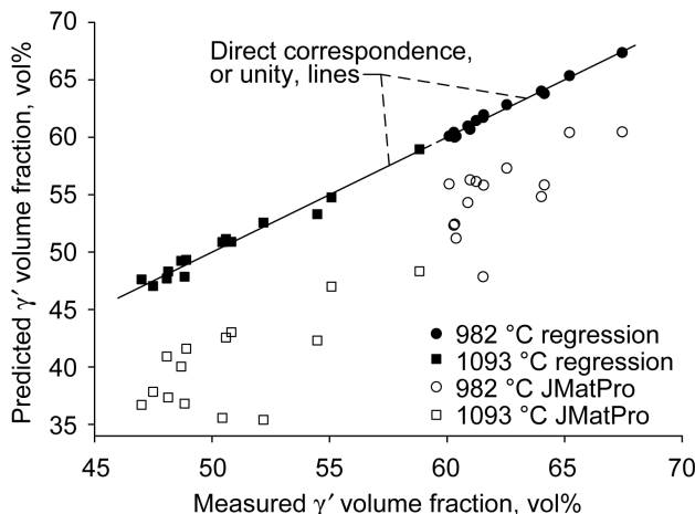
Figure 9.—Predicted versus measured \gamma' volume fractions are shown at 982 and 1093 °C. The solid symbols in the figure show the excellent fit obtained by the regression models developed in this study. The open symbols demonstrate that the JMatPro predictions consistently underpredicted the measured \gamma' volume fractions.
