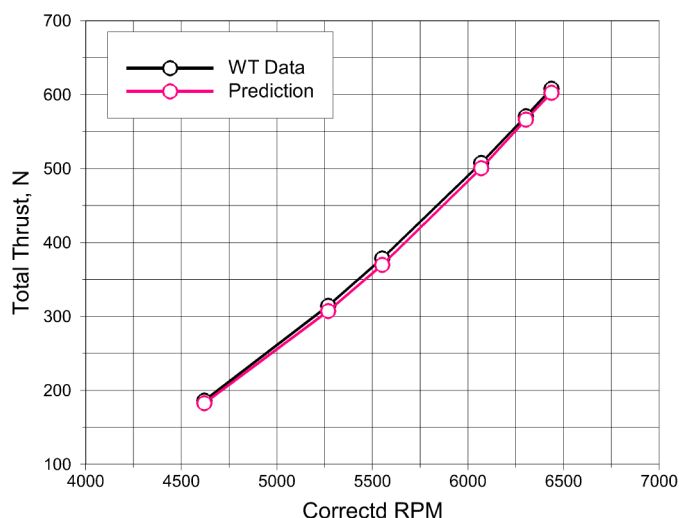
Figure 5.—Measured and predicted F31/A31 rotor thrust. Combined thrust produced by both rotors is plotted.
