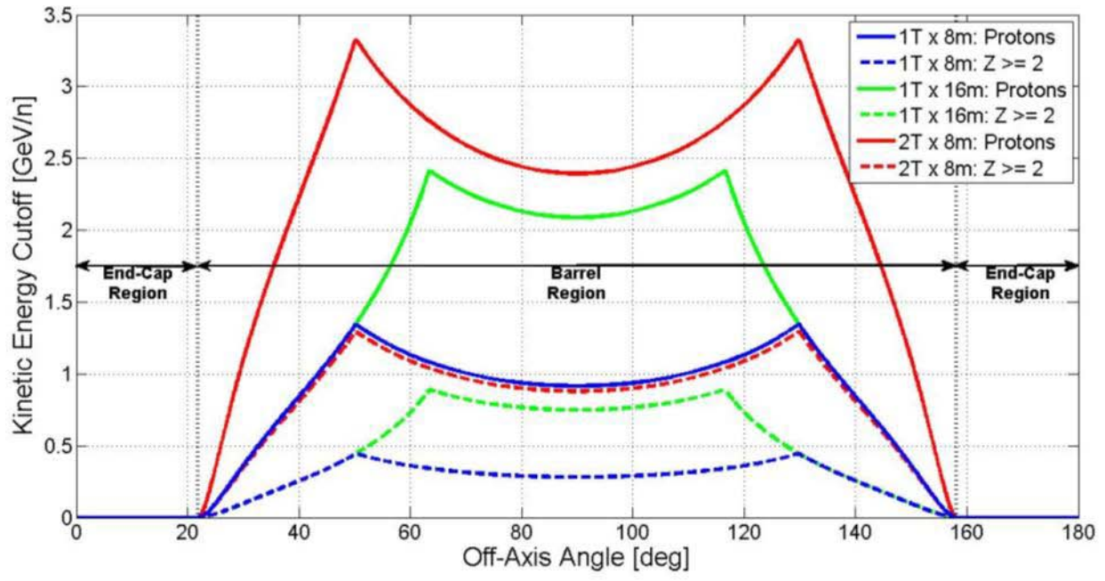
Figure 8.18. Open-Ended Cylinder Cutoff Energy at the Center of the Habitat ( r_i = 4\text{m} )
