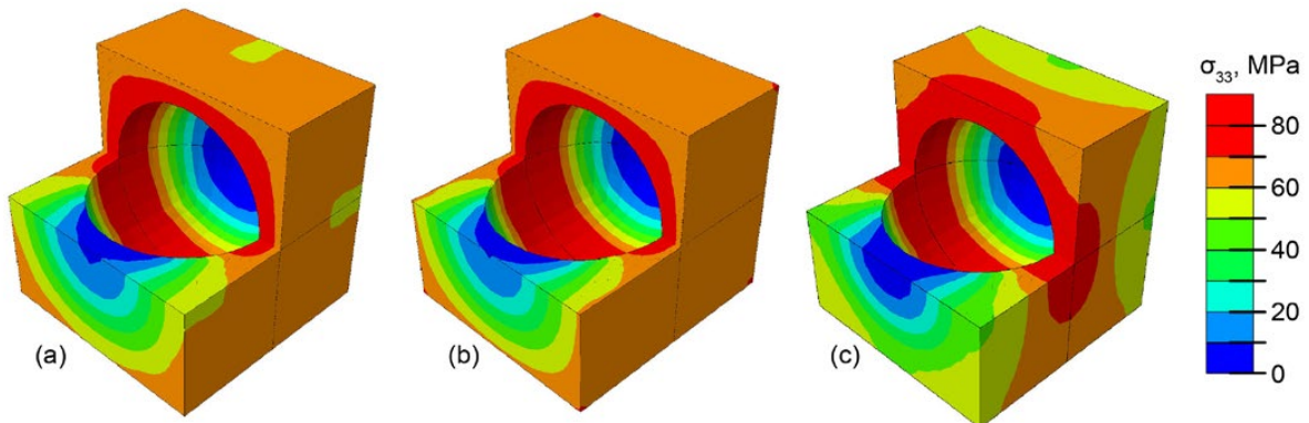
Figure 4.—Stress distributions in the RUC with a spherical cavity. (a) HFGMC results (periodic displacements), (b) FE results (periodic displacements), and (c) HFGMC results (periodic displacements and tractions).
