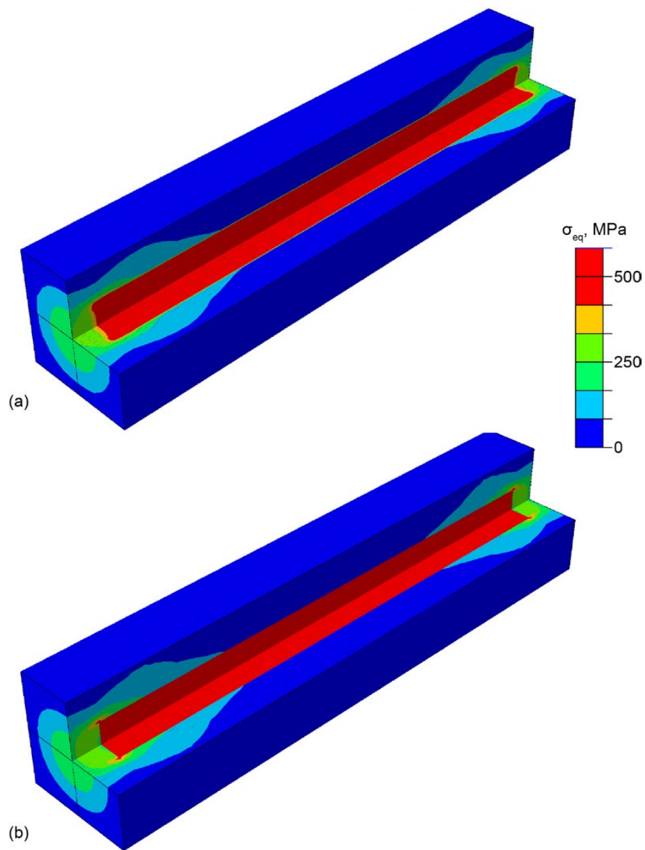
Figure 10.—Stress distributions in the RUC with the discontinuous fiber. (a) HFGMC results, (b) FE results.
