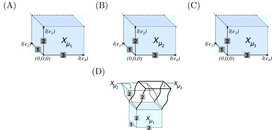
Figure 3. (A-C) The continuous state spaces X_{\mu_1}, X_{\mu_2}, X_{\mu_3} corresponding to discrete modes \mu_1, \mu_2, \mu_3 from Fig. ??. Among the discrete modes the system may enter from \mu_1 are \mu_2 and \mu_3 , accordingly as agent 2 enters e_2 or e_3 . Conflicting states not shown. (D) A gluing of X_{\mu_1} to X_{\mu_2} and to X_{\mu_3} . Glued, all three state spaces share a face, but no two have any other points in common. Conflicting states not shown.
