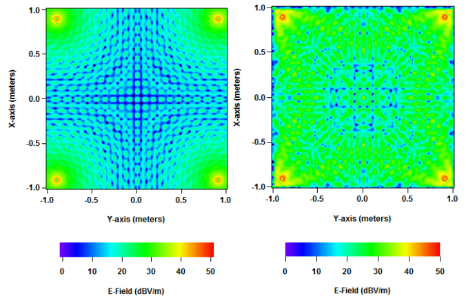
Figure 10. Electric field distributions for four Wi-Fi devices placed in free space (Left) and placed in a confined environment near the corners (Right).
