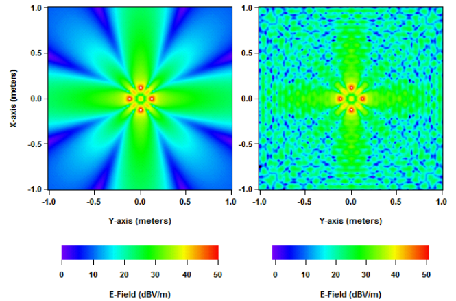
Figure 9. Electric field distributions for four Wi-Fi devices placed in free space (Left) and placed in a confined environment near the center (Right).
