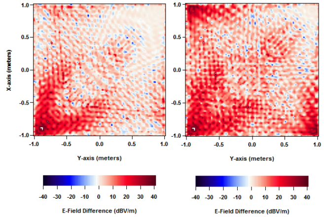
Figure 8. Electric field increases with multiple Wi-Fi devices as shown for two (Left) and four devices (Right).
