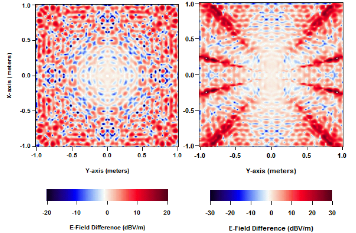
Figure 4. Differences of electric fields between in a confined space and in free space for one (Left) and two (Right) Wi-Fi devices.
