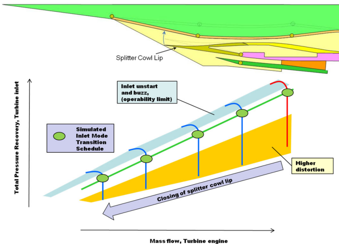
Figure 12.—Schematic plot of mode transition sequence representative of low-speed inlet test data.
