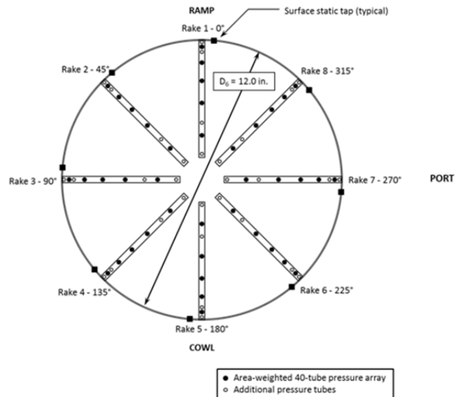
Figure 8.—Low-speed AIP rake array.
