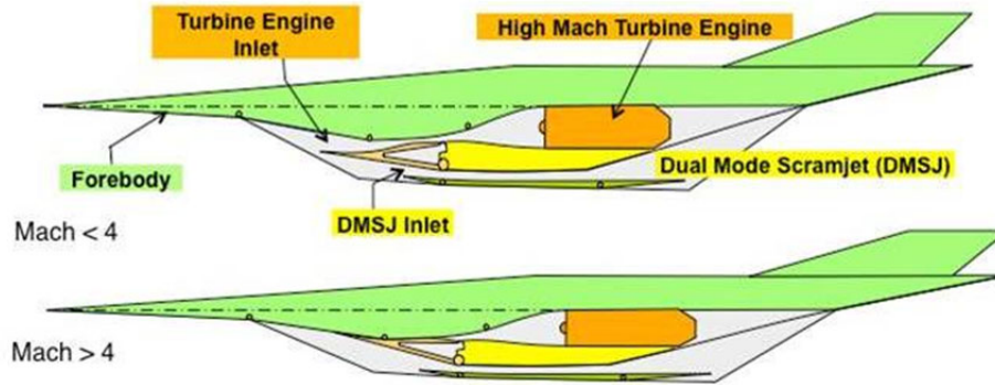
Figure 2.—Operating modes of the TBCC propulsion system.
