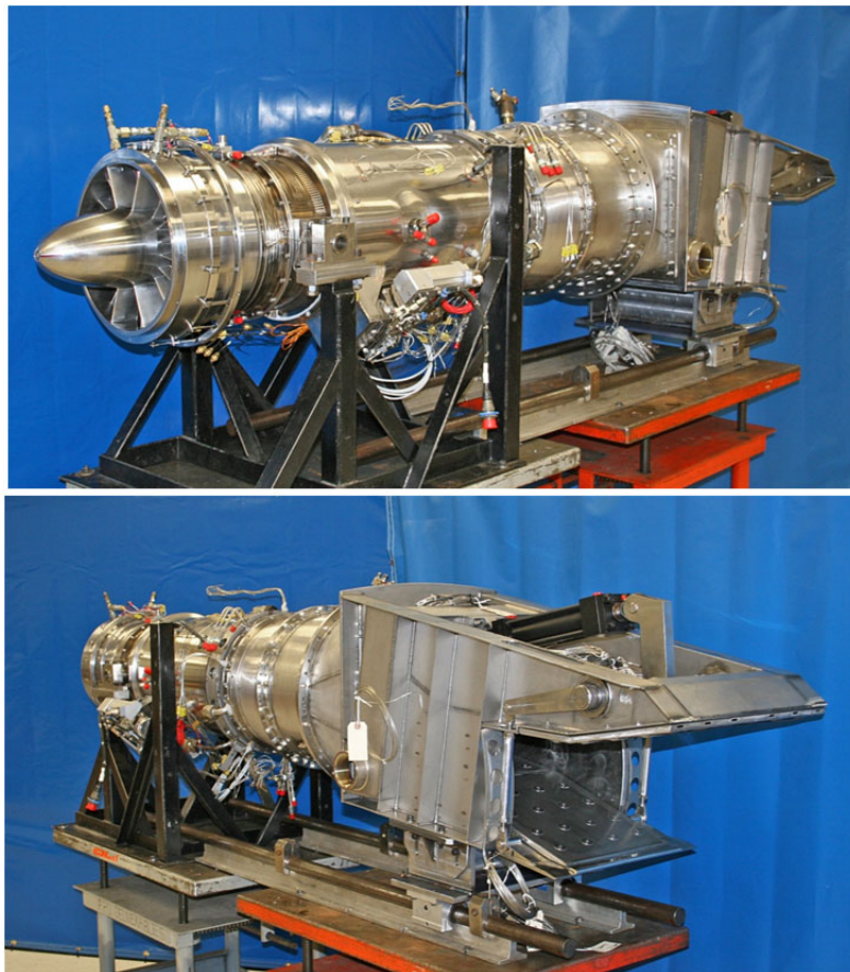
Figure 11.—Williams International High Mach WJ38 turbine engine and integrated nozzle assembly.
