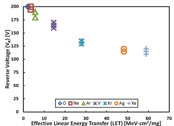
Fig. 3. The last voltage at which an ON Semiconductor MBR20200CT diode was irradiated without destructive failure. The error bars (many of which are smaller than the symbols) indicate the voltage at which the part did fail.
