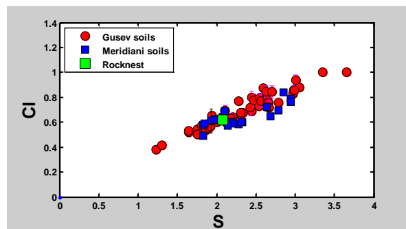
Figure 3: Consistent trend in Cl versus S for soils analyzed by MER and Curiosity APXS instruments (values in wt%).
