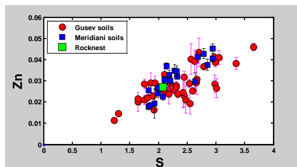
Fig. 4: Correlation of Zn and S (values in wt%).
