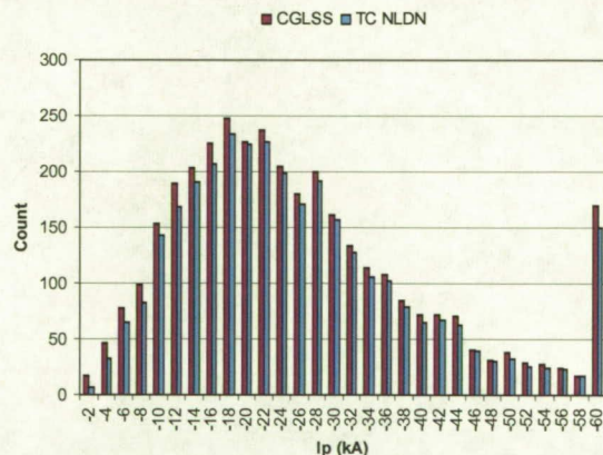
Figure 6b Number of CGLSS strokes (red) and time-correlated NLDN strokes (blue) as a function of I_p ( 2 \text{ kA} < |I_p| < 100 \text{ kA} ).
