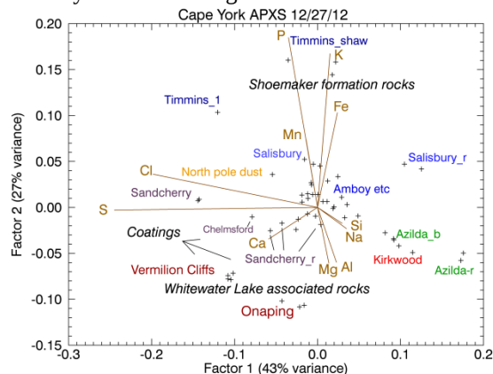
Fig. 5 – CA for Cape York rocks, where b=brushed and r=ratted. The Azilda series are for Whitewater Lake outcrops whereas Sandcherry and Chelmsford are for overlying coatings (arrow shows coatings trend).
