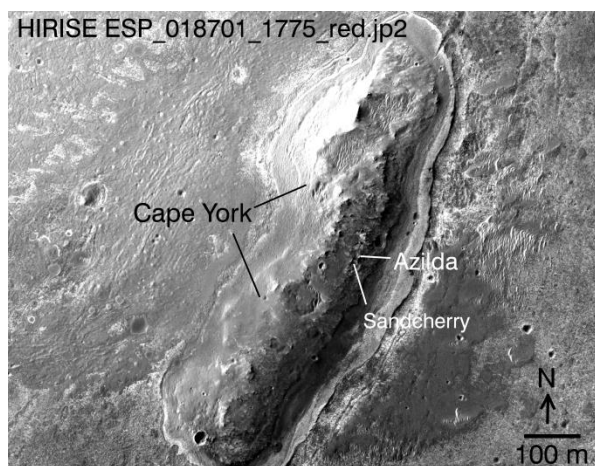
Fig. 1 – HiRISE view of Cape York, an isolated Endeavour crater rim segment. Sandcherry and Azilda are in-situ targets that are part of the Matijevic Hill portion of Cape York examined during Opportunity’s “walk about”.
