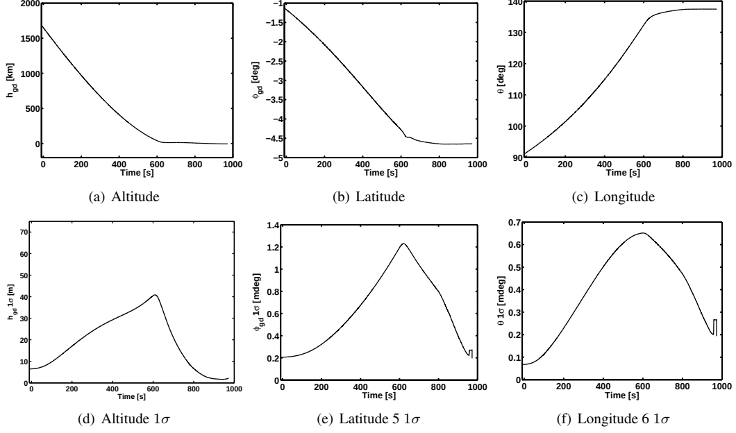
Figure 11. Position Estimates
