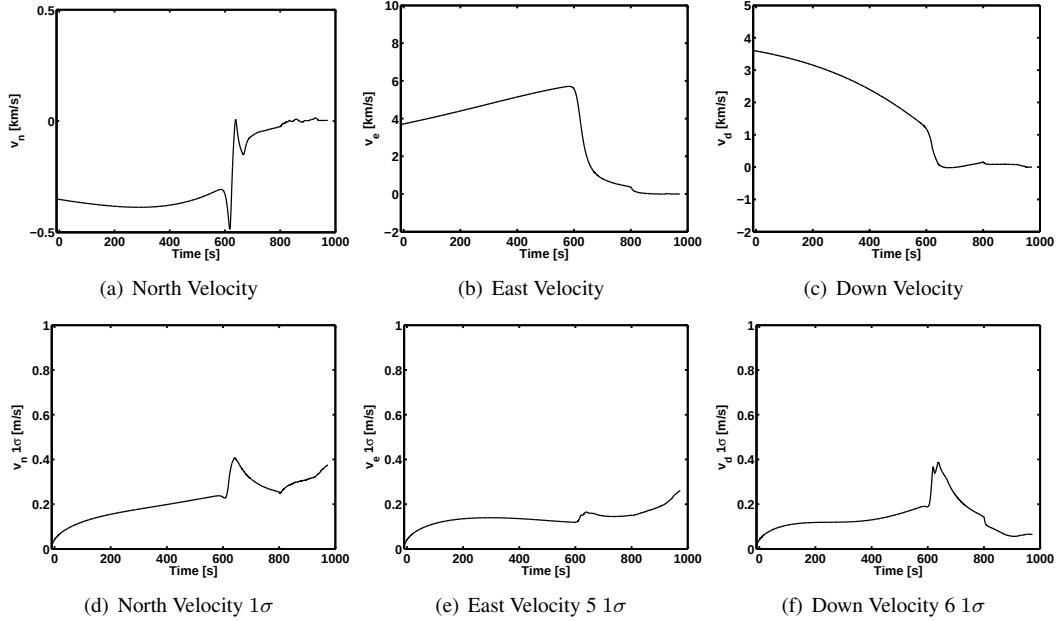
Figure 12. Velocity Estimates
