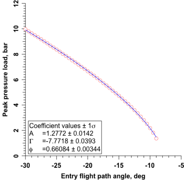
Figure 6. Variation with EFPA of peak pressure load for m_E = 2000 kg and 11.6 km/s entry velocity. The open symbols are 3DoF predictions and the line is a curve fit of the form shown in Eq. 6.
