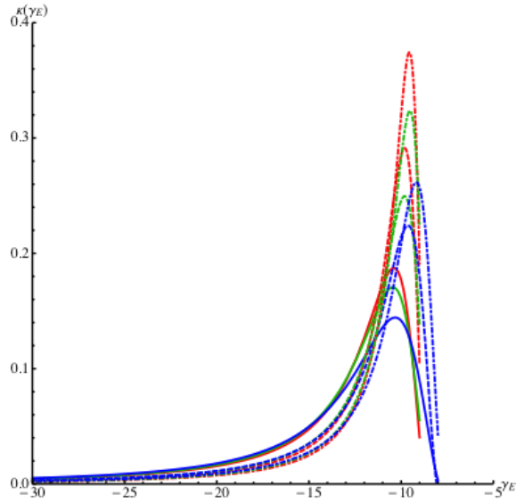
Figure 10. Variation with EFPA of curvature (Eq. 4) of total heat load distributions for m_E = 2000 kg and nine V_E - \beta_E combinations (10.8, 11.2, and 11.6 km/s and 2.5, 3.5, and 4.5 m diameter).
