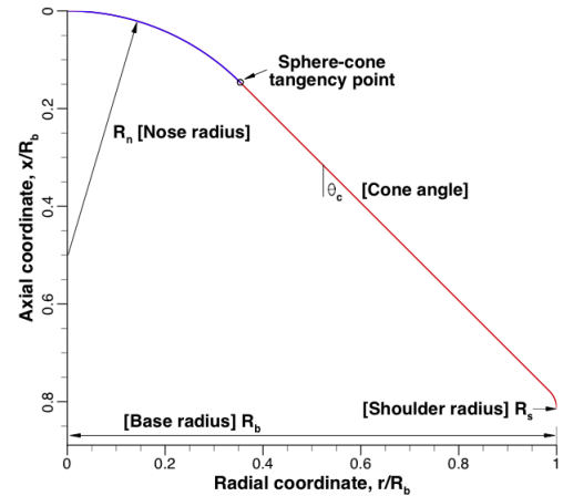
Figure 2. Geometry of a sphere-cone heatshield. The axisymmetric geometry is described by four parameters – (i) base radius, R_b , (ii) spherical nose radius, R_n , (iii) a toroidal shoulder radius, R_s , and (iv) the cone half angle, \theta_c .
