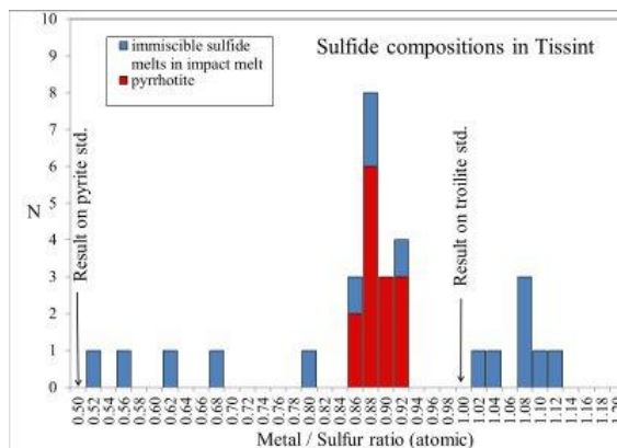
Fig. 1b. Histogram of metal/S ratios in Tissint sulfides.
