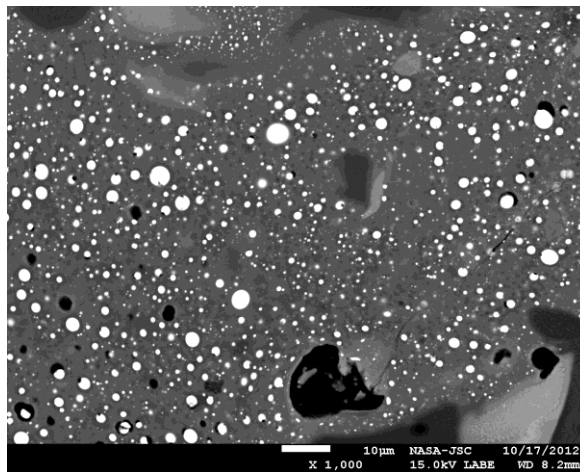
Fig. 2a. BSE image of abundant sulfide droplets in a large melt pocket in EETA79001,507.
