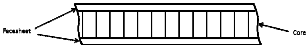
Figure 3. Typical cross-sectional view of a sandwich composite.
