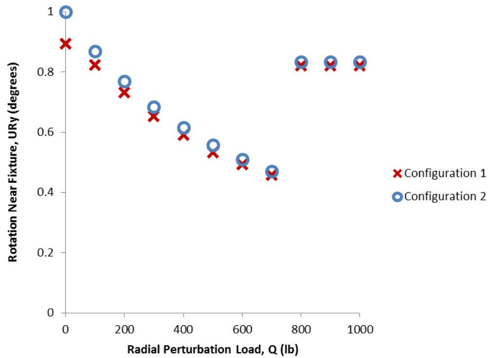
Figure 15. The tangential rotation near fixtures plotted versus the radial perturbation load.
