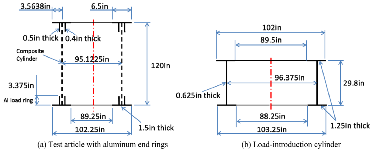
Figure 5. Geometry of (a) the test article with aluminum end rings, and (b) a load-introduction cylinder
