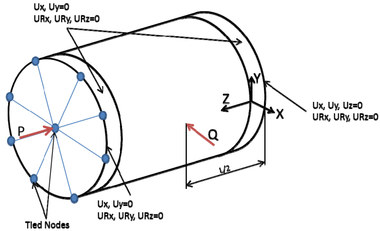
Figure 6. Sketch of the configuration 1 test article with boundary and loading conditions applied to 3.4-in. potted region of the test article.
