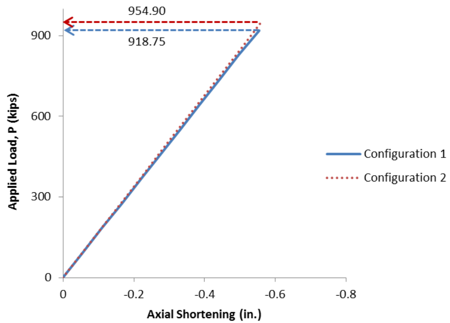
Figure 9. Applied load versus axial shortening from the nonlinear analyses.
