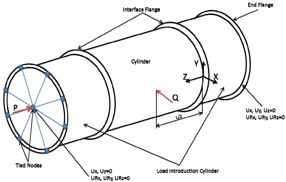
Figure 7. Sketch of the configuration 2 assembly with the test cylinder and load introduction rings.
