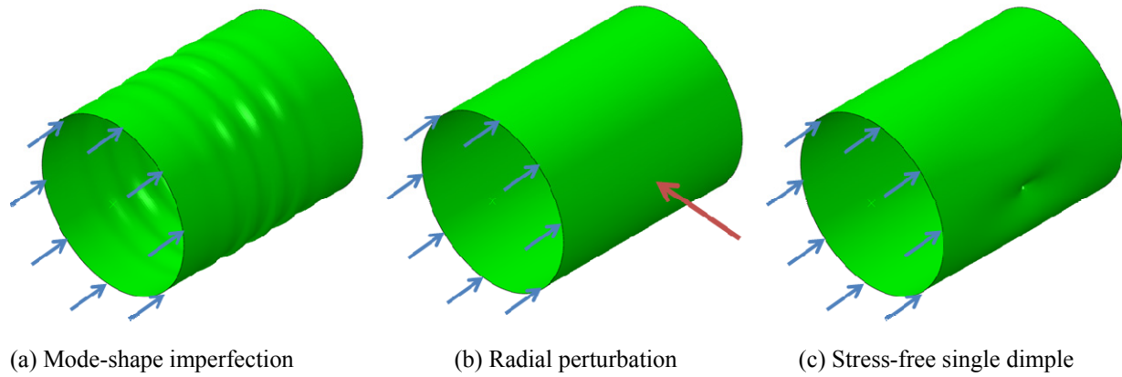
Figure 1. Three ways to introduce geometrical imperfections: (a) mode-shape imperfection, (b) radial perturbation load, and (c) stress-free single dimple.
