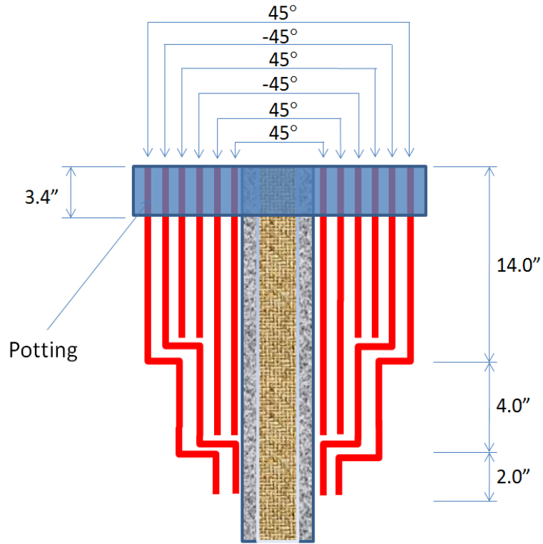
Figure 4. Cross-sectional schematic of the pad-up region of the test article.
